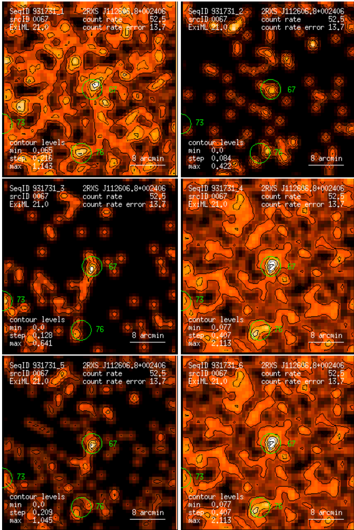
Figure 67: RASS 931731: detection 0067: band rate images, Gaussian filter: (1) PSPC channels 11 – 41, (2) 52 – 90, (3) 91 – 201, (4) 11 – 235, (5) 52 – 201, (6) 11 – 201. Broad band rates in counts/ks. Band rate contour levels in counts/ks/arcmin 2 .
