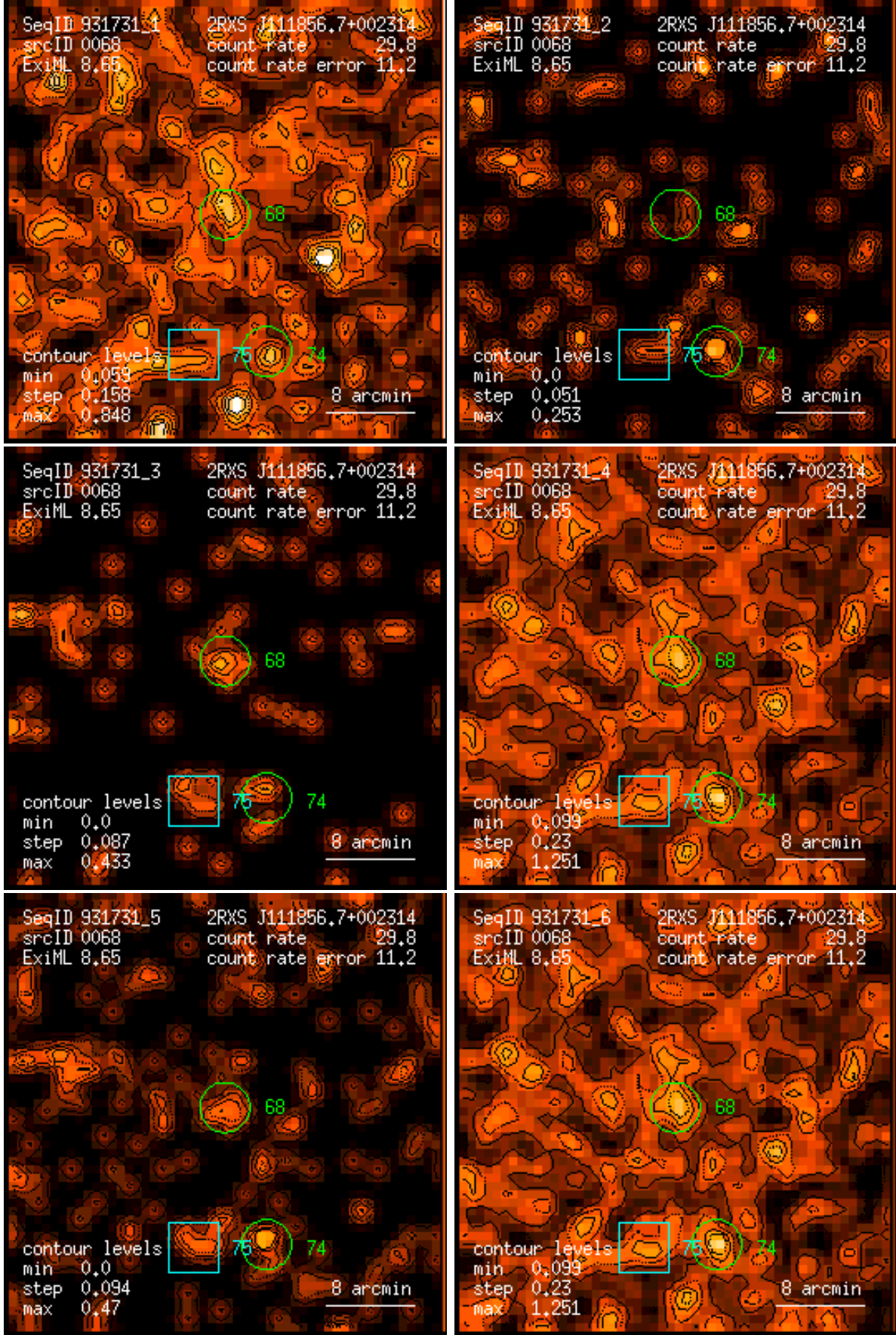
Figure 68: RASS 931731: detection 0068: band rate images, Gaussian filter: (1) PSPC channels 11 – 41, (2) 52 – 90, (3) 91 – 201, (4) 11 – 235, (5) 52 – 201, (6) 11 – 201. Broad band rates in counts/ks. Band rate contour levels in counts/ks/arcmin 2 .
