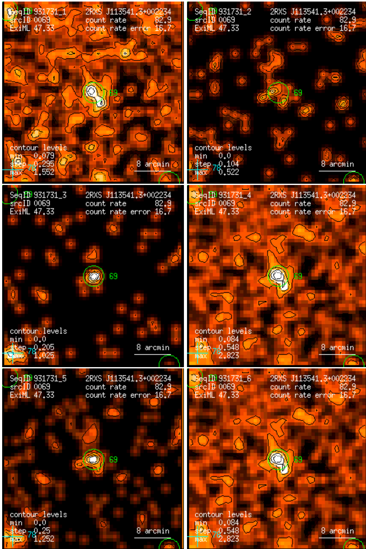
Figure 69: RASS 931731: detection 0069: band rate images, Gaussian filter: (1) PSPC channels 11 – 41, (2) 52 – 90, (3) 91 – 201, (4) 11 – 235, (5) 52 – 201, (6) 11 – 201. Broad band rates in counts/ks. Band rate contour levels in counts/ks/arcmin 2 .
