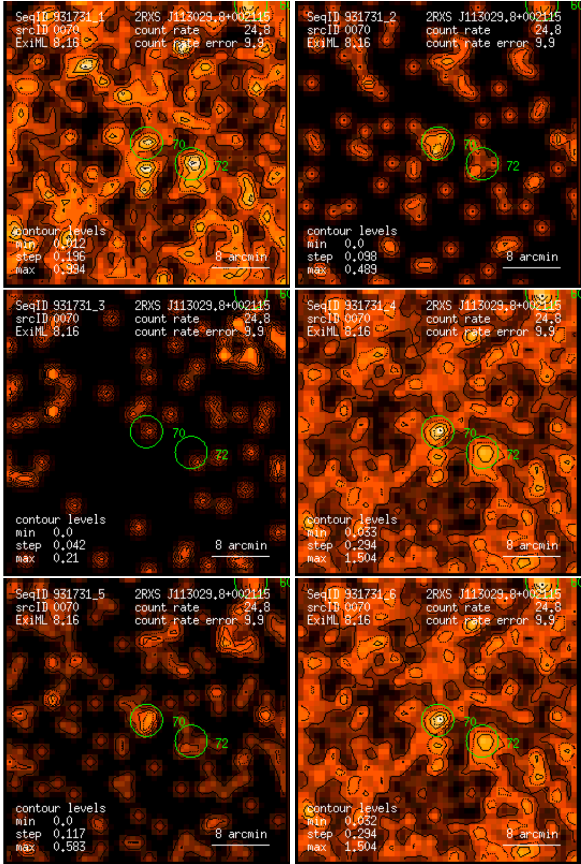
Figure 70: RASS 931731: detection 0070: band rate images, Gaussian filter: (1) PSPC channels 11 – 41, (2) 52 – 90, (3) 91 – 201, (4) 11 – 235, (5) 52 – 201, (6) 11 – 201. Broad band rates in counts/ks. Band rate contour levels in counts/ks/arcmin 2 .
