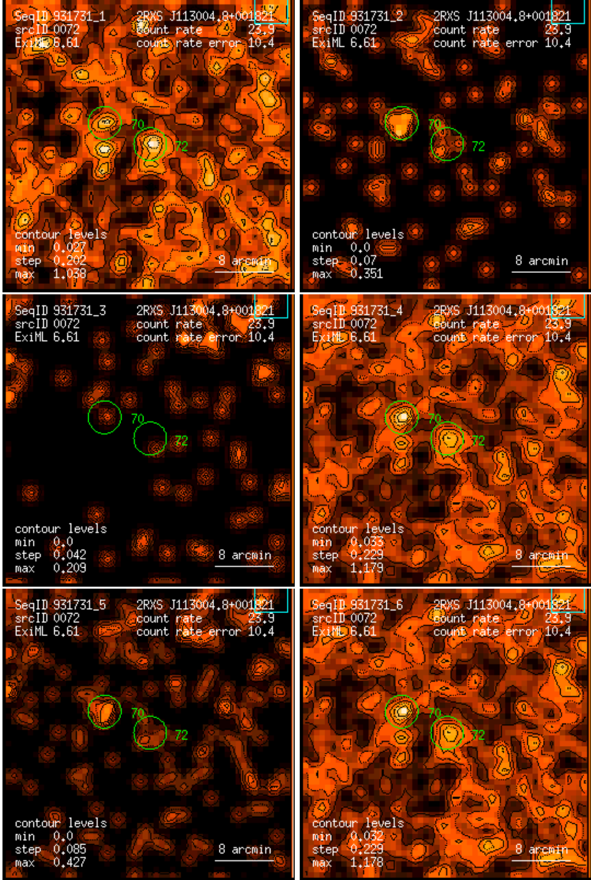
Figure 72: RASS 931731: detection 0072: band rate images, Gaussian filter: (1) PSPC channels 11 – 41, (2) 52 – 90, (3) 91 – 201, (4) 11 – 235, (5) 52 – 201, (6) 11 – 201. Broad band rates in counts/ks. Band rate contour levels in counts/ks/arcmin 2 .
