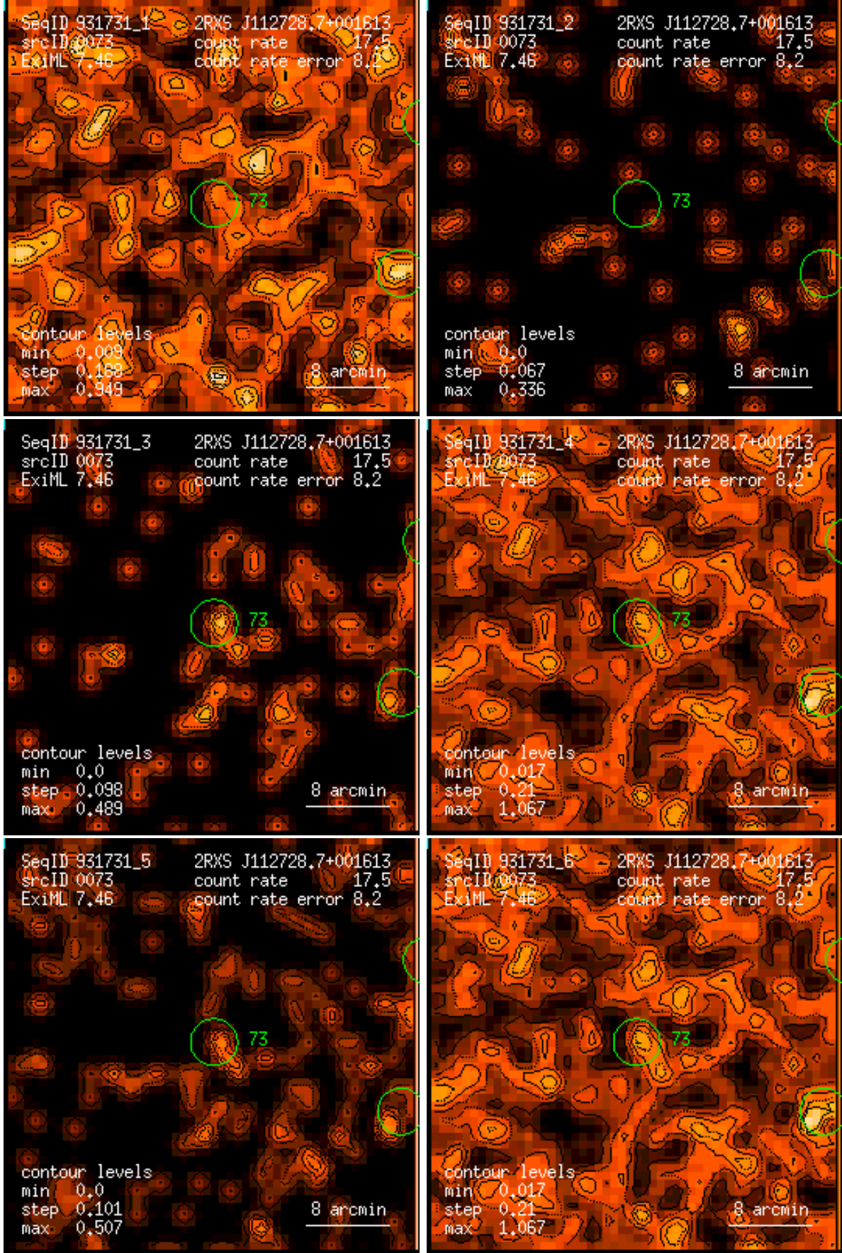
Figure 73: RASS 931731: detection 0073: band rate images, Gaussian filter: (1) PSPC channels 11 – 41, (2) 52 – 90, (3) 91 – 201, (4) 11 – 235, (5) 52 – 201, (6) 11 – 201. Broad band rates in counts/ks. Band rate contour levels in counts/ks/arcmin 2 .
