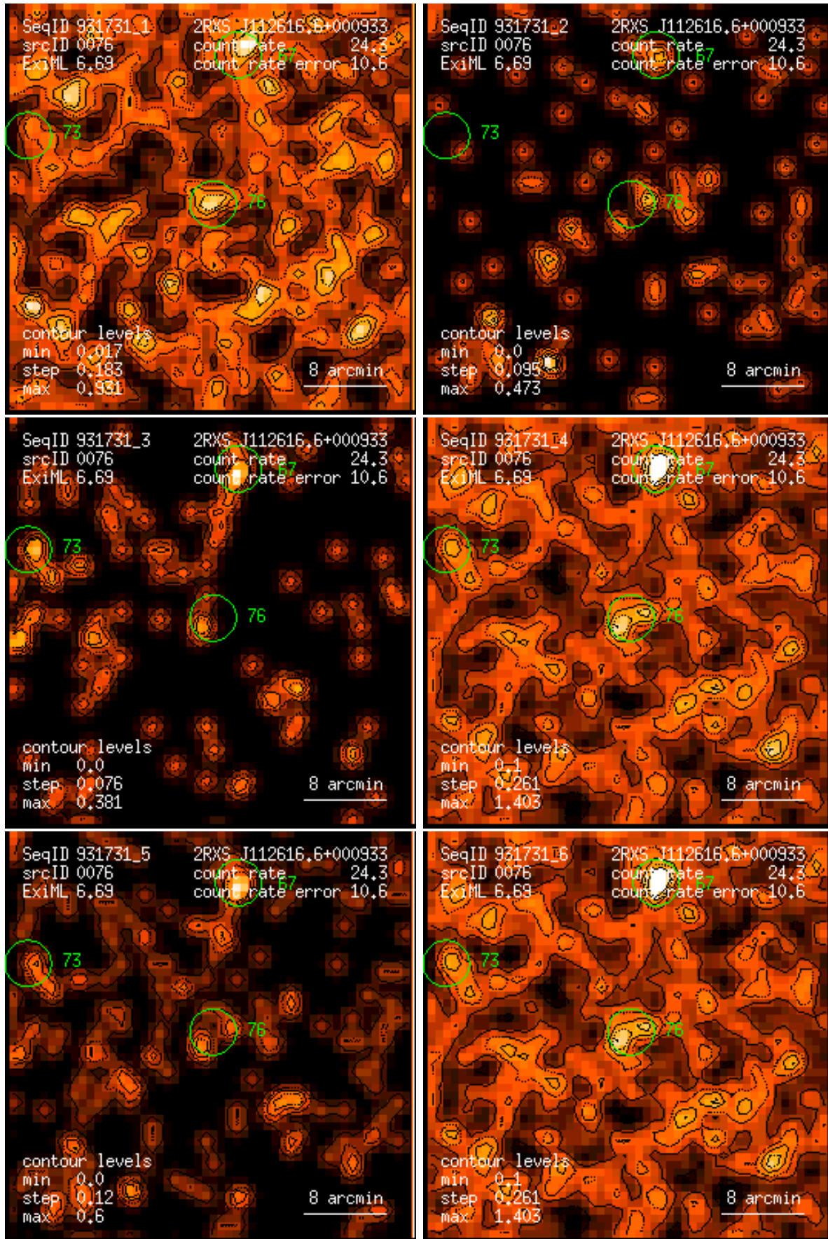
Figure 76: RASS 931731: detection 0076: band rate images, Gaussian filter: (1) PSPC channels 11 – 41, (2) 52 – 90, (3) 91 – 201, (4) 11 – 235, (5) 52 – 201, (6) 11 – 201. Broad band rates in counts/ks. Band rate contour levels in counts/ks/arcmin 2 .
