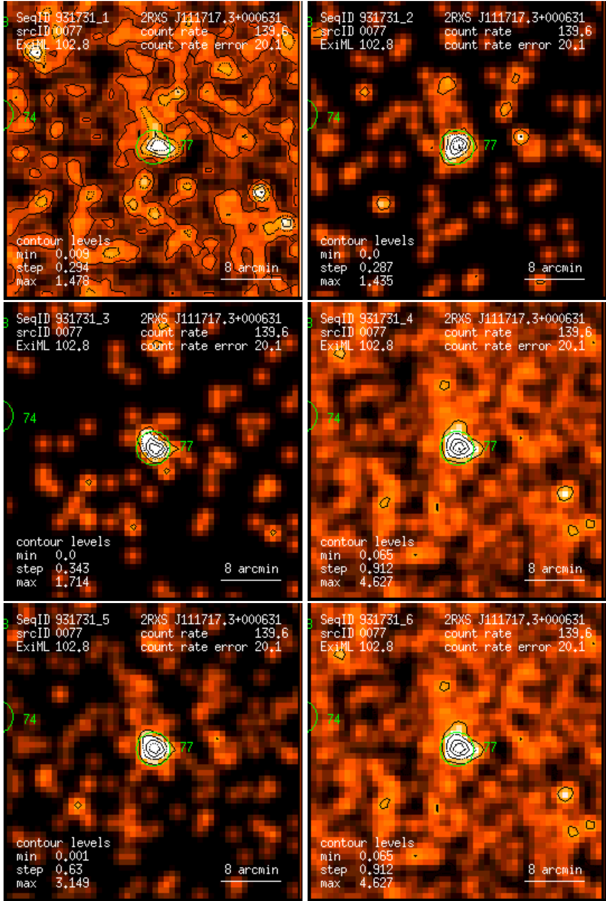
Figure 77: RASS 931731: detection 0077: band rate images, Gaussian filter: (1) PSPC channels 11 – 41, (2) 52 – 90, (3) 91 – 201, (4) 11 – 235, (5) 52 – 201, (6) 11 – 201. Broad band rates in counts/ks. Band rate contour levels in counts/ks/arcmin 2 .
