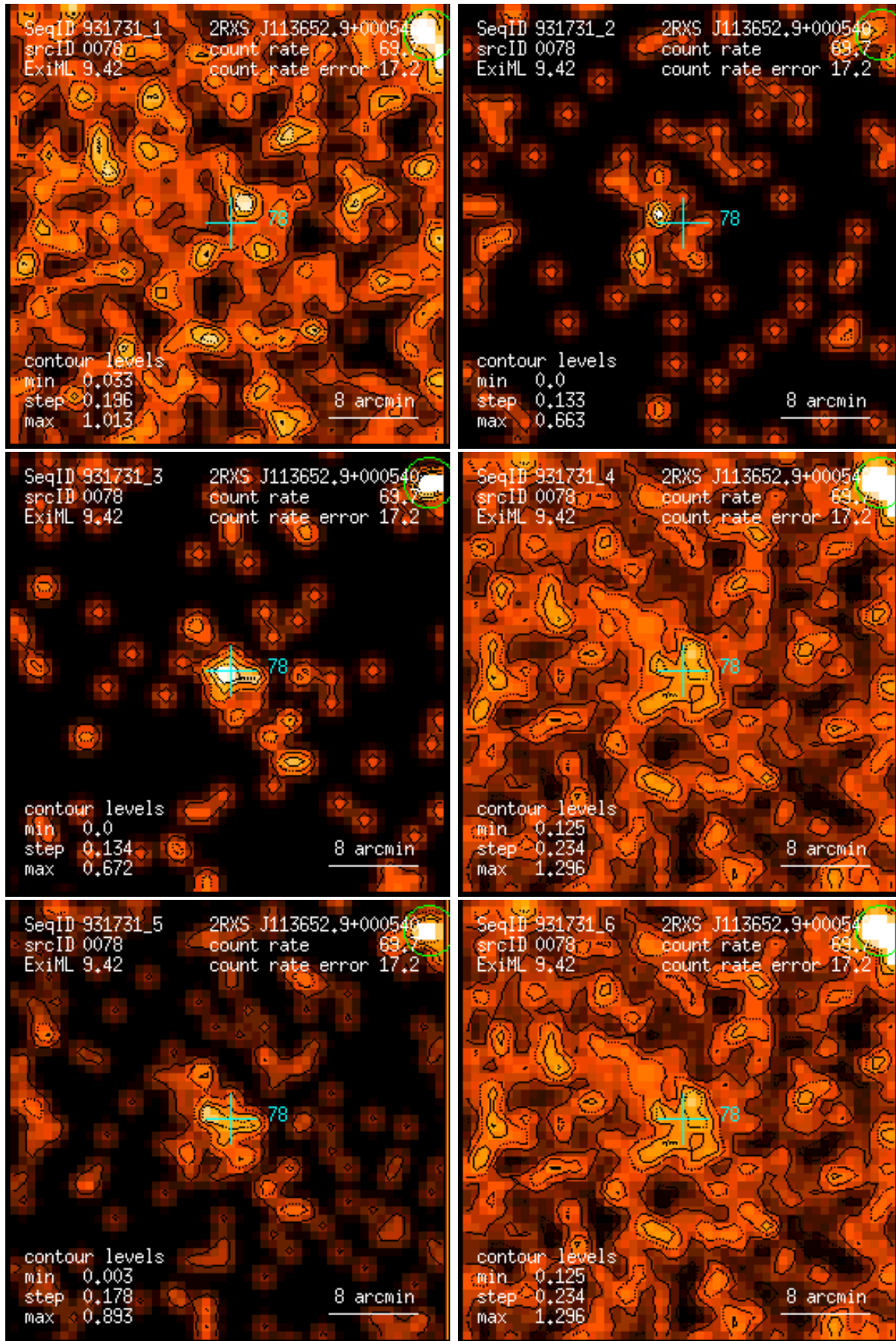
Figure 78: RASS 931731: detection 0078: band rate images, Gaussian filter: (1) PSPC channels 11 – 41, (2) 52 – 90, (3) 91 – 201, (4) 11 – 235, (5) 52 – 201, (6) 11 – 201. Broad band rates in counts/ks. Band rate contour levels in counts/ks/arcmin 2 .
