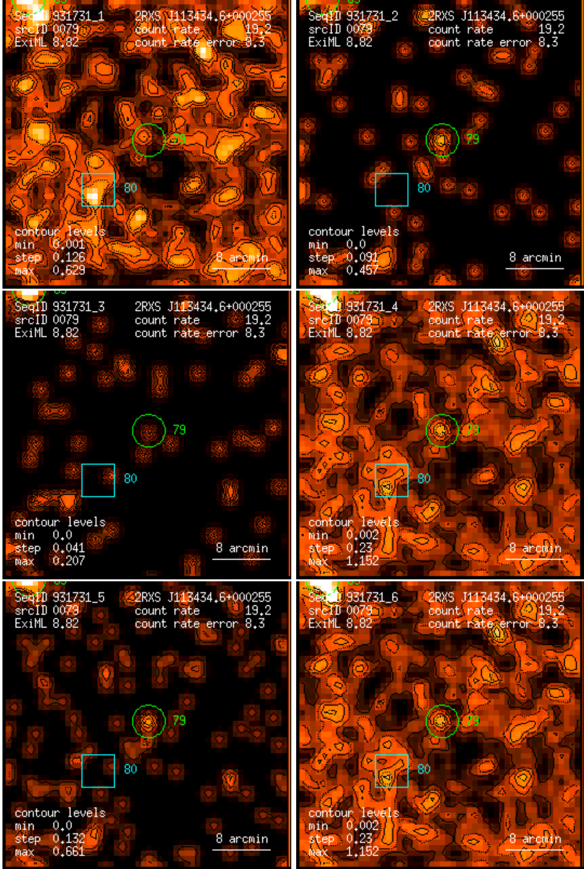
Figure 79: RASS 931731: detection 0079: band rate images, Gaussian filter: (1) PSPC channels 11 – 41, (2) 52 – 90, (3) 91 – 201, (4) 11 – 235, (5) 52 – 201, (6) 11 – 201. Broad band rates in counts/ks. Band rate contour levels in counts/ks/arcmin 2 .
