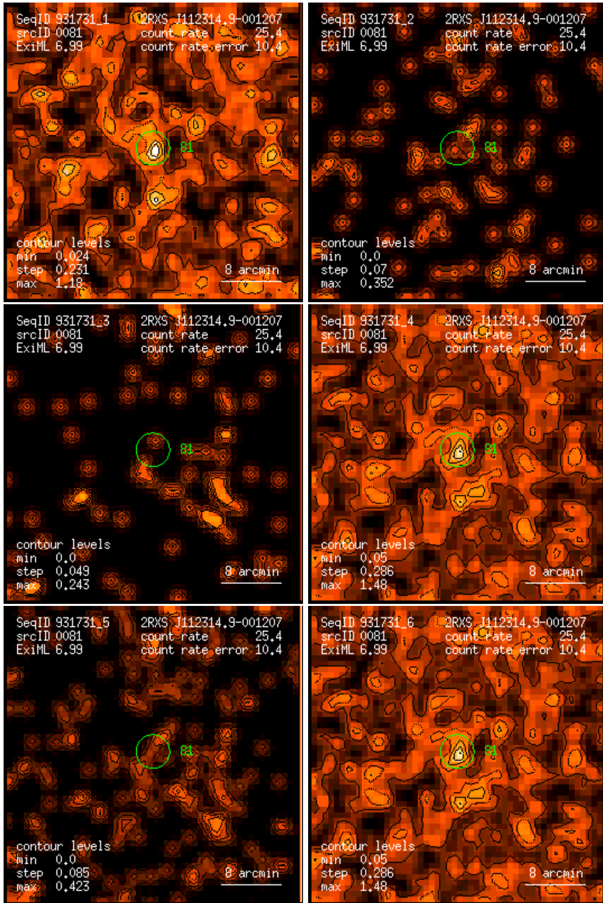
Figure 81: RASS 931731: detection 0081: band rate images, Gaussian filter: (1) PSPC channels 11 – 41, (2) 52 – 90, (3) 91 – 201, (4) 11 – 235, (5) 52 – 201, (6) 11 – 201. Broad band rates in counts/ks. Band rate contour levels in counts/ks/arcmin 2 .
