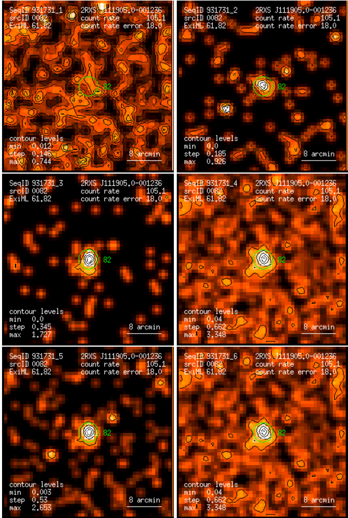
Figure 82: RASS 931731: detection 0082: band rate images, Gaussian filter: (1) PSPC channels 11 – 41, (2) 52 – 90, (3) 91 – 201, (4) 11 – 235, (5) 52 – 201, (6) 11 – 201. Broad band rates in counts/ks. Band rate contour levels in counts/ks/arcmin 2 .
