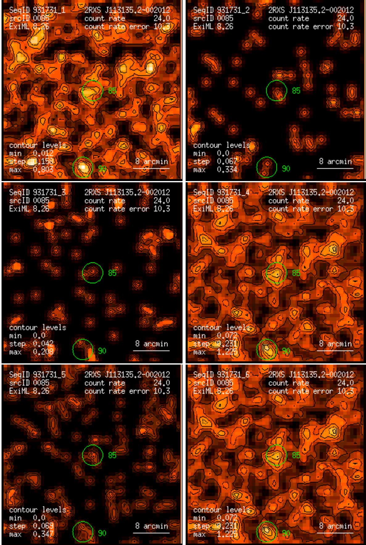
Figure 85: RASS 931731: detection 0085: band rate images, Gaussian filter: (1) PSPC channels 11 – 41, (2) 52 – 90, (3) 91 – 201, (4) 11 – 235, (5) 52 – 201, (6) 11 – 201. Broad band rates in counts/ks. Band rate contour levels in counts/ks/arcmin 2 .
