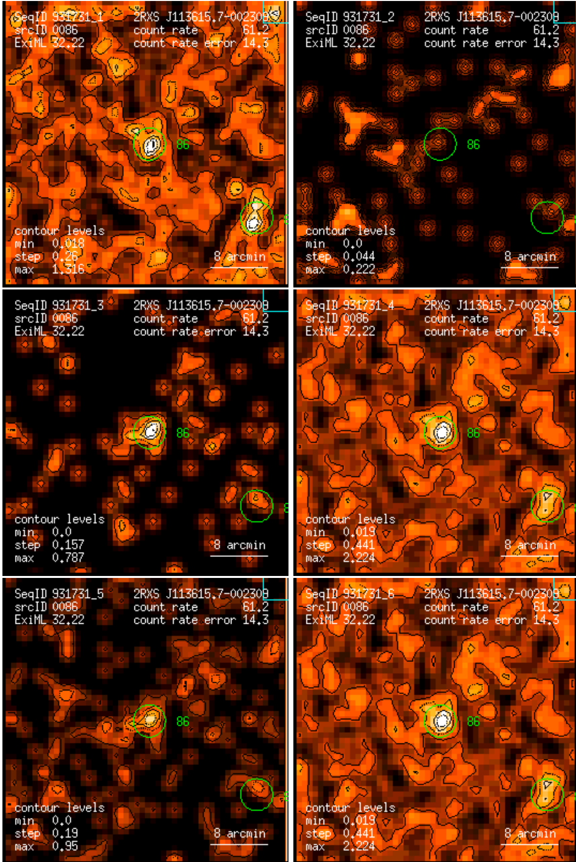
Figure 86: RASS 931731: detection 0086: band rate images, Gaussian filter: (1) PSPC channels 11 – 41, (2) 52 – 90, (3) 91 – 201, (4) 11 – 235, (5) 52 – 201, (6) 11 – 201. Broad band rates in counts/ks. Band rate contour levels in counts/ks/arcmin 2 .
