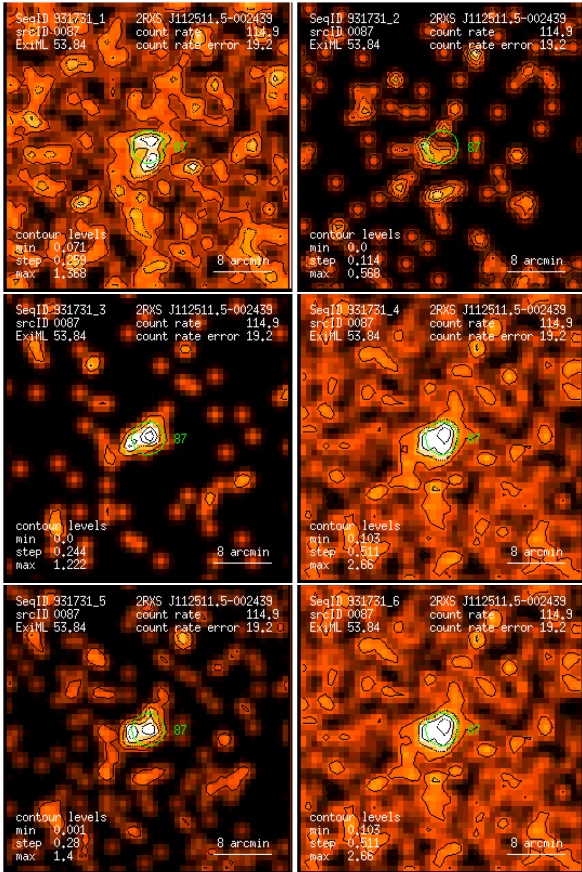
Figure 87: RASS 931731: detection 0087: band rate images, Gaussian filter: (1) PSPC channels 11 – 41, (2) 52 – 90, (3) 91 – 201, (4) 11 – 235, (5) 52 – 201, (6) 11 – 201. Broad band rates in counts/ks. Band rate contour levels in counts/ks/arcmin 2 .
