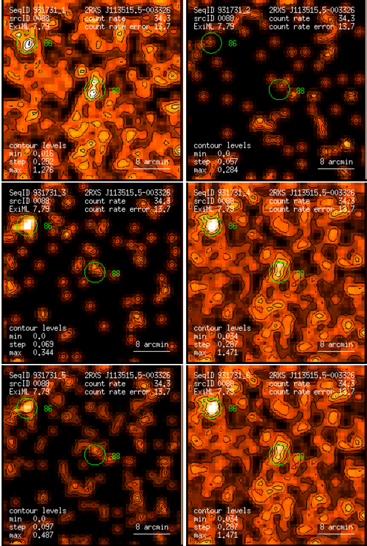
Figure 88: RASS 931731: detection 0088: band rate images, Gaussian filter: (1) PSPC channels 11 – 41, (2) 52 – 90, (3) 91 – 201, (4) 11 – 235, (5) 52 – 201, (6) 11 – 201. Broad band rates in counts/ks. Band rate contour levels in counts/ks/arcmin 2 .
