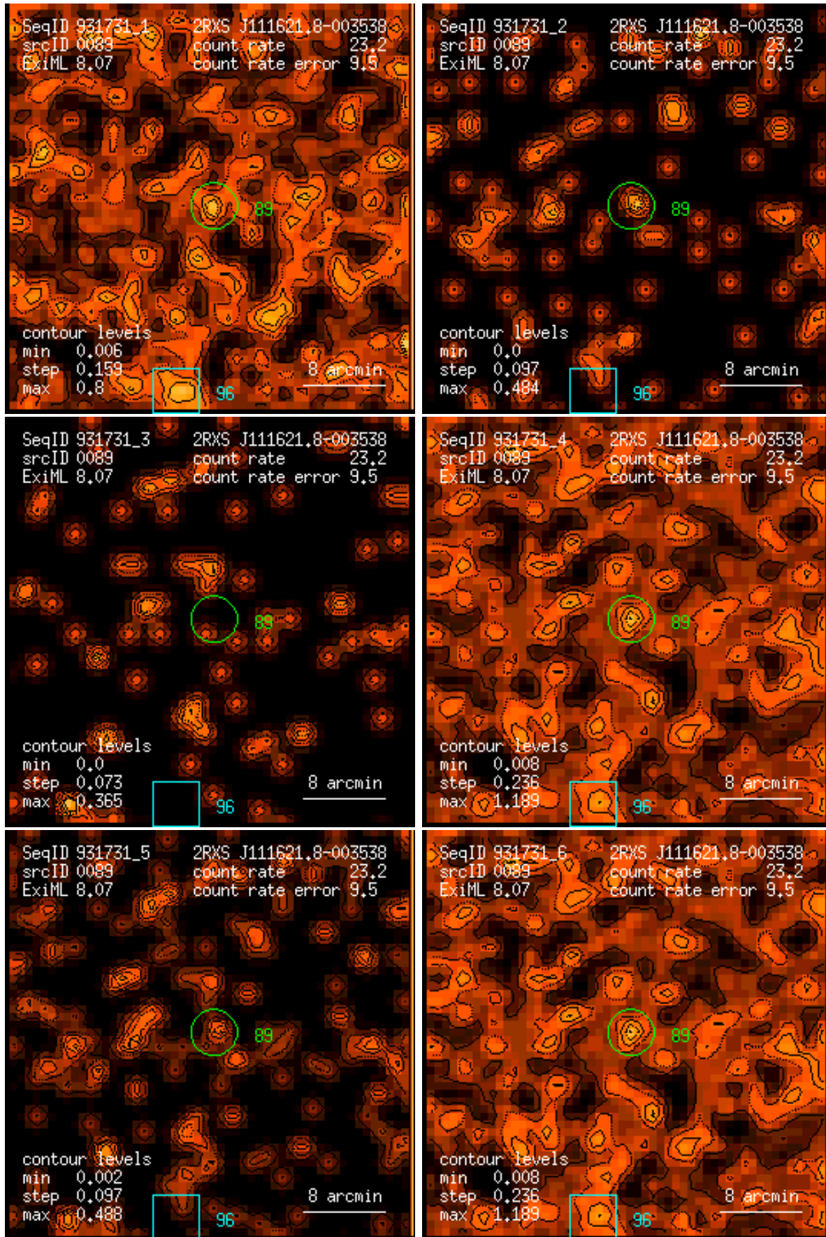
Figure 89: RASS 931731: detection 0089: band rate images, Gaussian filter: (1) PSPC channels 11 – 41, (2) 52 – 90, (3) 91 – 201, (4) 11 – 235, (5) 52 – 201, (6) 11 – 201. Broad band rates in counts/ks. Band rate contour levels in counts/ks/arcmin 2 .
