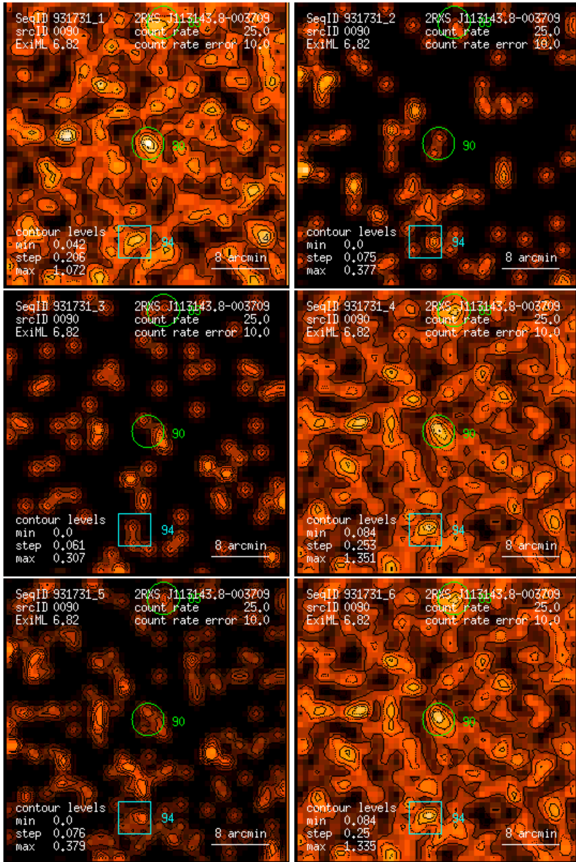
Figure 90: RASS 931731: detection 0090: band rate images, Gaussian filter: (1) PSPC channels 11 – 41, (2) 52 – 90, (3) 91 – 201, (4) 11 – 235, (5) 52 – 201, (6) 11 – 201. Broad band rates in counts/ks. Band rate contour levels in counts/ks/arcmin 2 .
