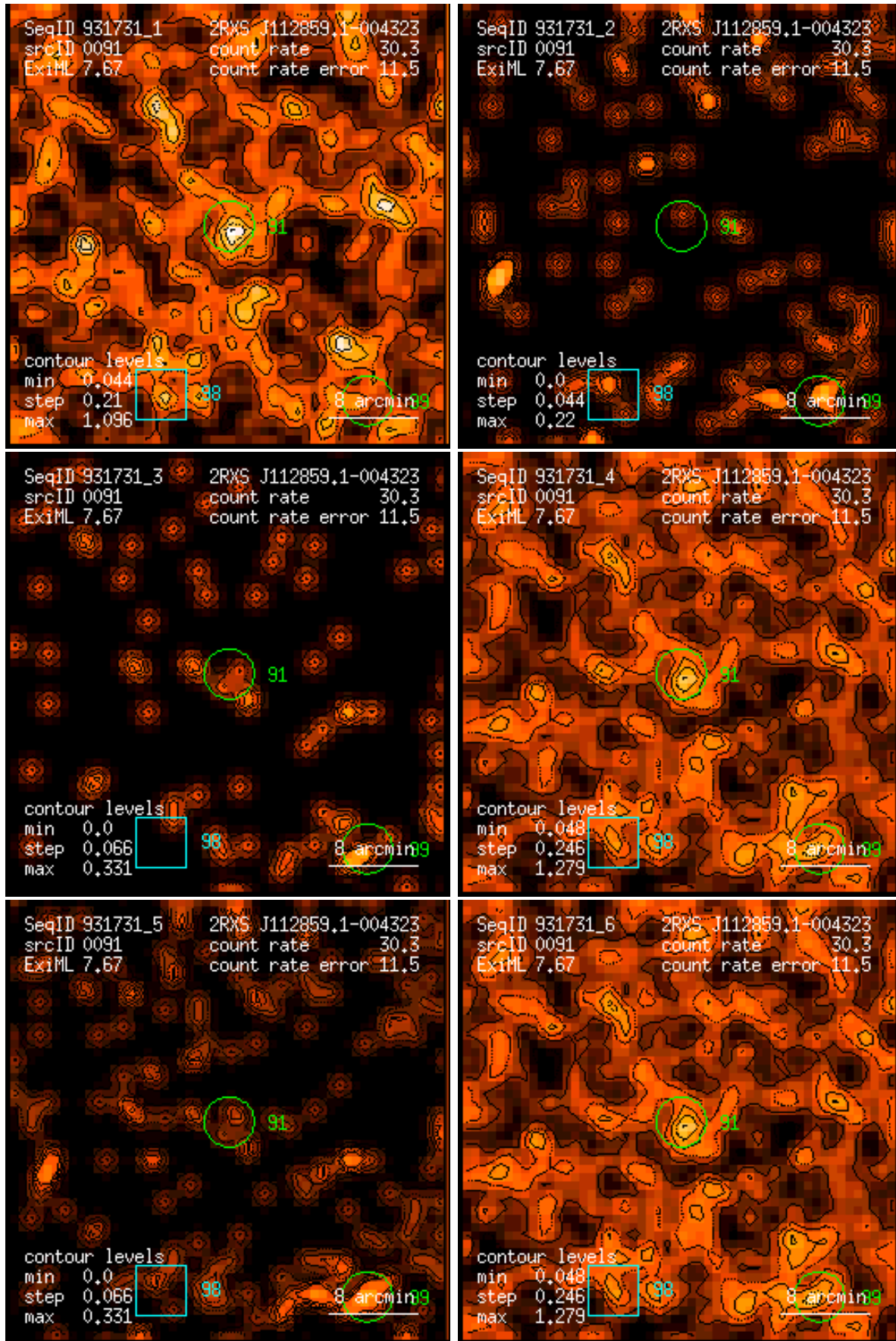
Figure 91: RASS 931731: detection 0091: band rate images, Gaussian filter: (1) PSPC channels 11 – 41, (2) 52 – 90, (3) 91 – 201, (4) 11 – 235, (5) 52 – 201, (6) 11 – 201. Broad band rates in counts/ks. Band rate contour levels in counts/ks/arcmin 2 .
