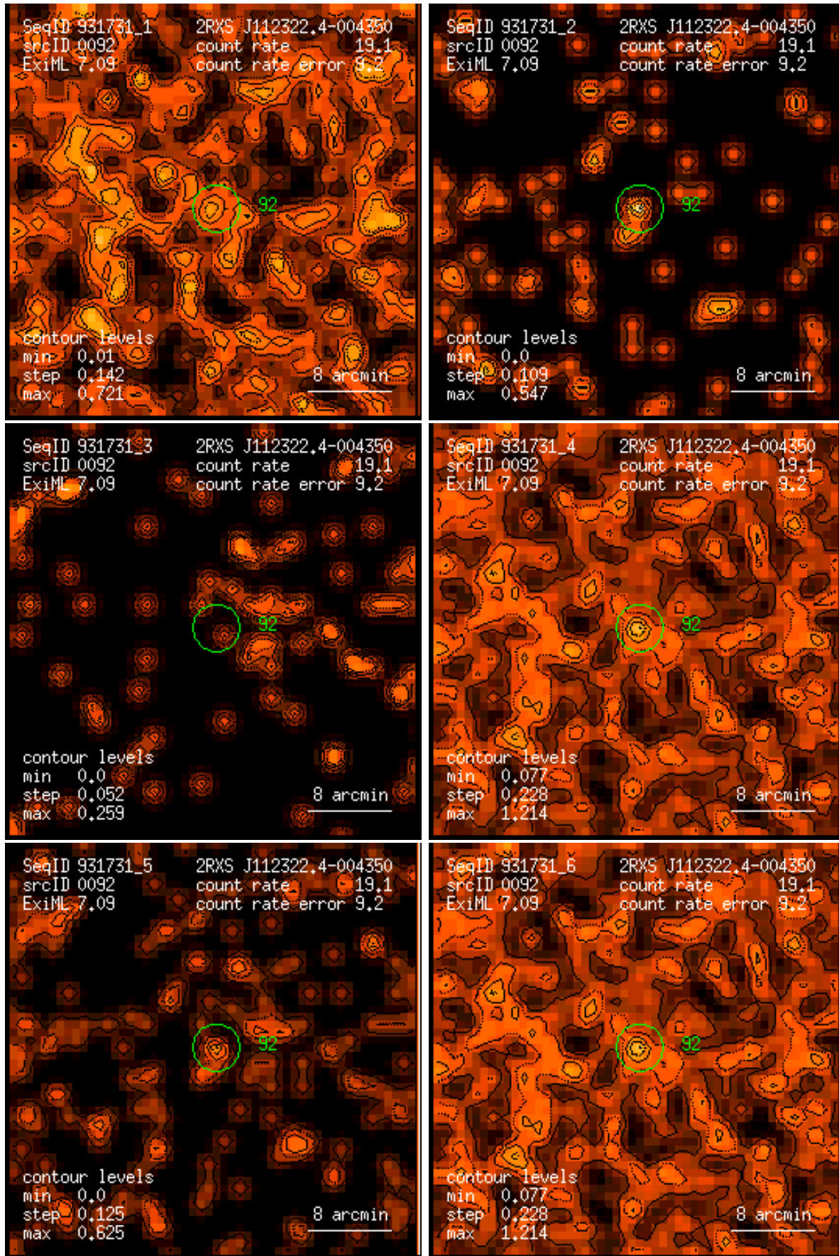
Figure 92: RASS 931731: detection 0092: band rate images, Gaussian filter: (1) PSPC channels 11 – 41, (2) 52 – 90, (3) 91 – 201, (4) 11 – 235, (5) 52 – 201, (6) 11 – 201. Broad band rates in counts/ks. Band rate contour levels in counts/ks/arcmin 2 .
