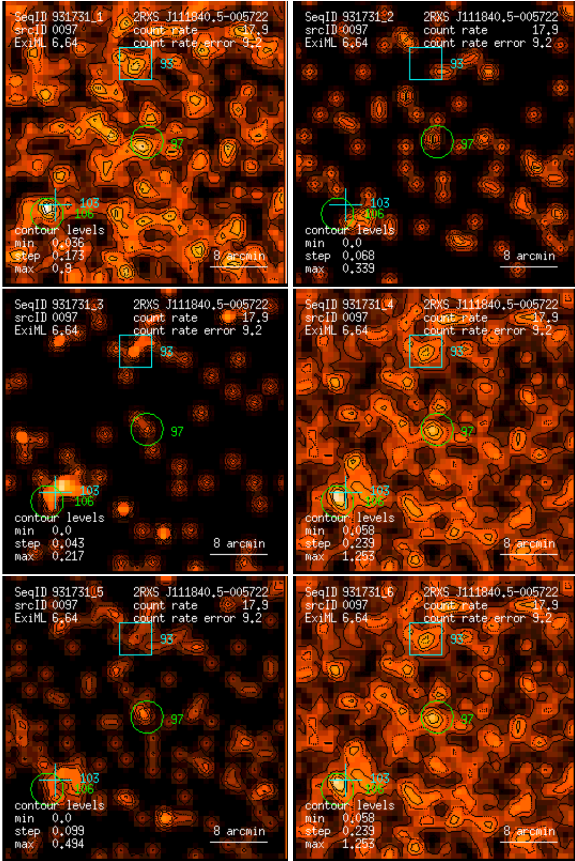
Figure 97: RASS 931731: detection 0097: band rate images, Gaussian filter: (1) PSPC channels 11 – 41, (2) 52 – 90, (3) 91 – 201, (4) 11 – 235, (5) 52 – 201, (6) 11 – 201. Broad band rates in counts/ks. Band rate contour levels in counts/ks/arcmin 2 .
