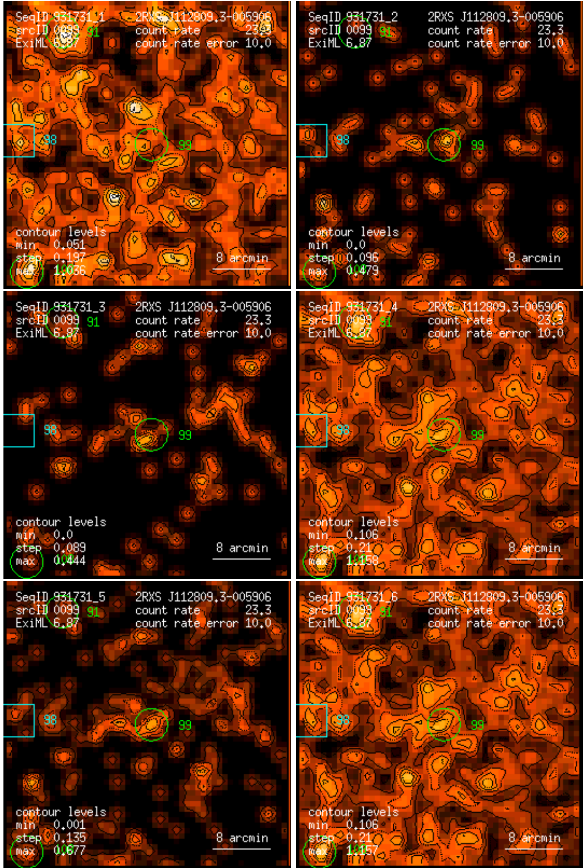
Figure 99: RASS 931731: detection 0099: band rate images, Gaussian filter: (1) PSPC channels 11 – 41, (2) 52 – 90, (3) 91 – 201, (4) 11 – 235, (5) 52 – 201, (6) 11 – 201. Broad band rates in counts/ks. Band rate contour levels in counts/ks/arcmin 2 .
