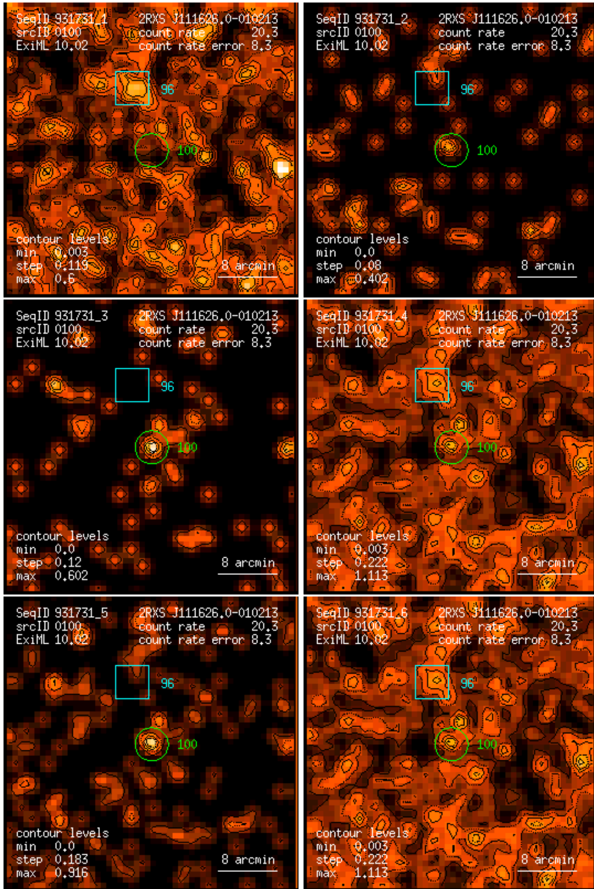
Figure 100: RASS 931731: detection 0100: band rate images, Gaussian filter: (1) PSPC channels 11 – 41, (2) 52 – 90, (3) 91 – 201, (4) 11 – 235, (5) 52 – 201, (6) 11 – 201. Broad band rates in counts/ks. Band rate contour levels in counts/ks/arcmin 2 .
