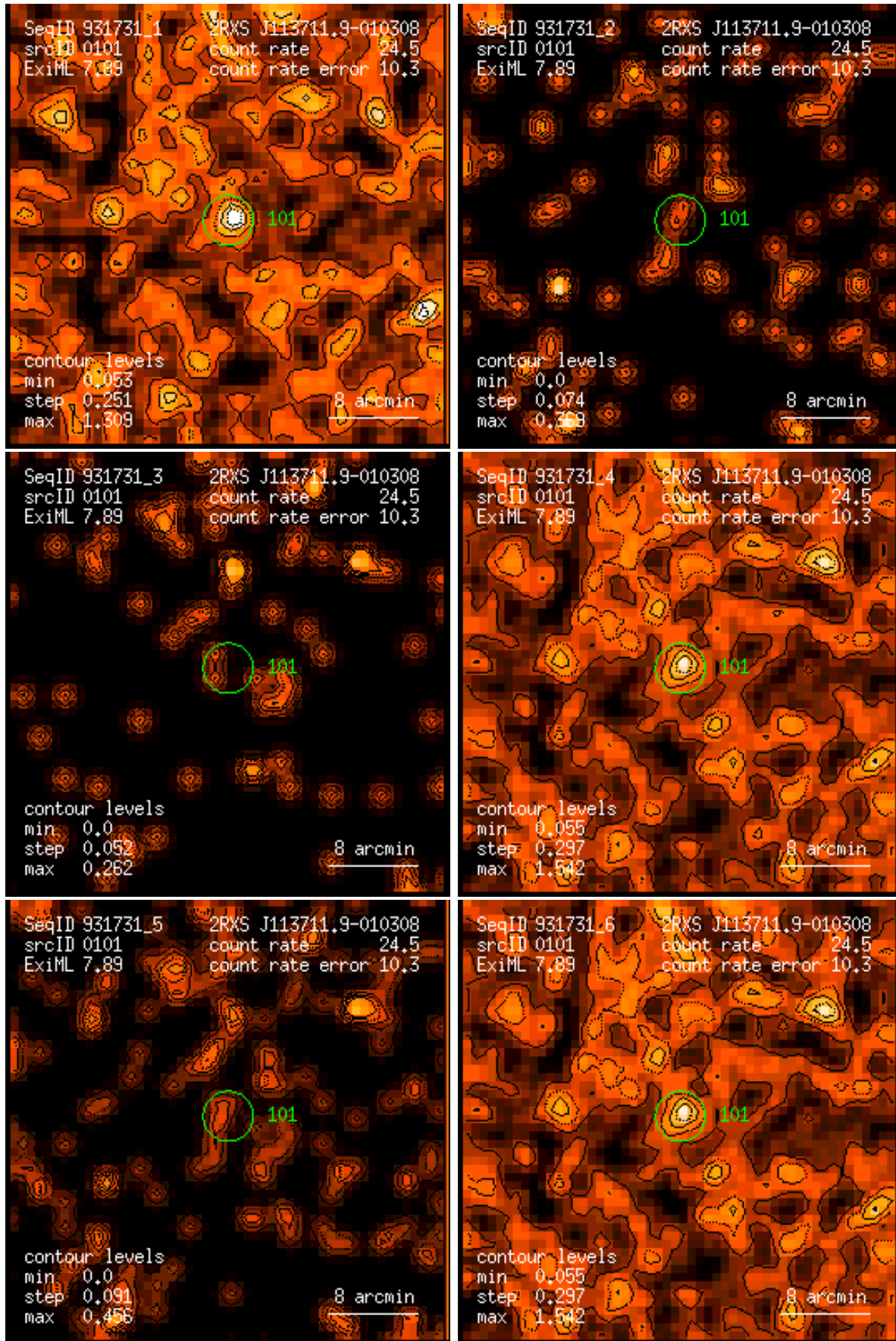
Figure 101: RASS 931731: detection 0101: band rate images, Gaussian filter: (1) PSPC channels 11 – 41, (2) 52 – 90, (3) 91 – 201, (4) 11 – 235, (5) 52 – 201, (6) 11 – 201. Broad band rates in counts/ks. Band rate contour levels in counts/ks/arcmin 2 .
