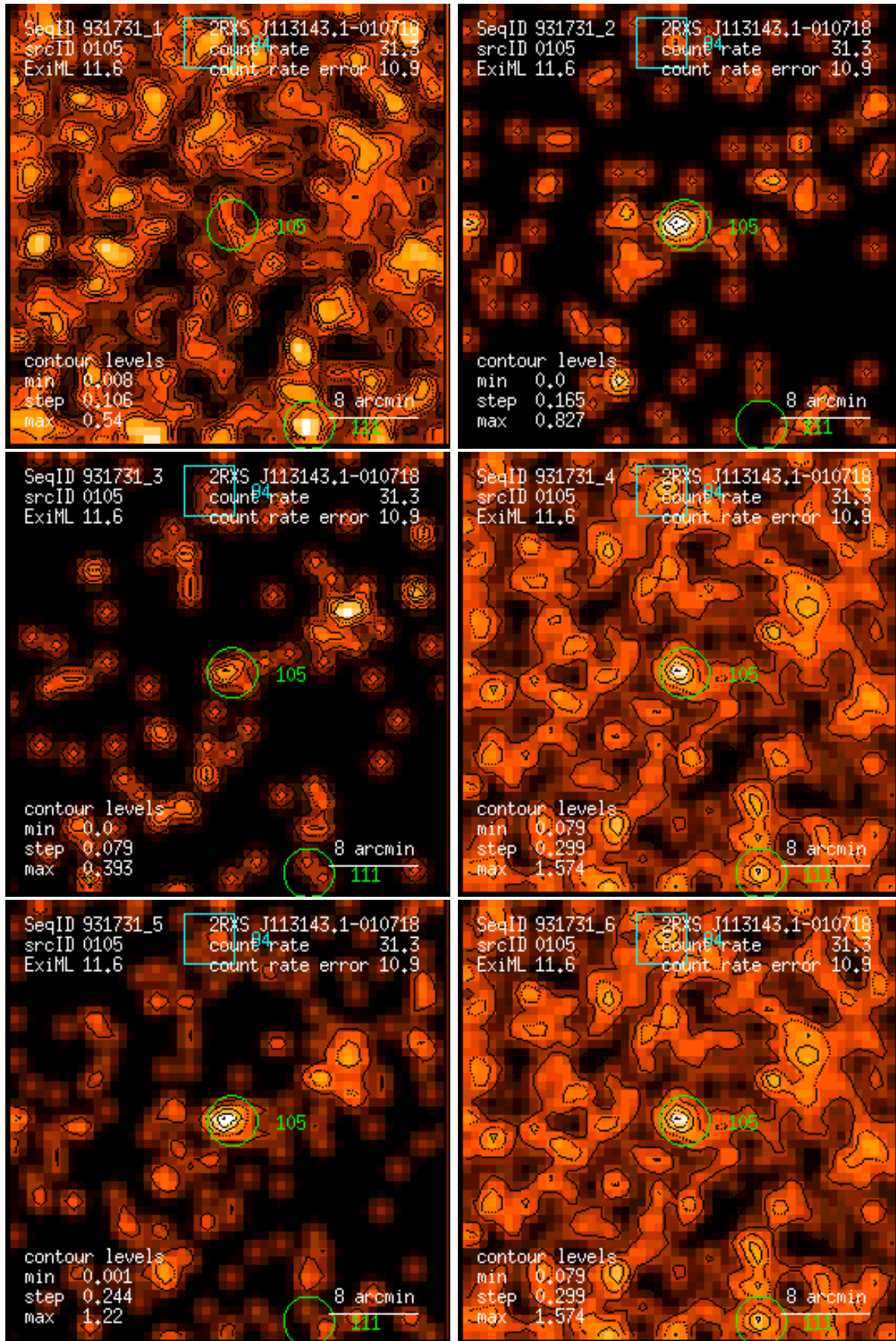
Figure 105: RASS 931731: detection 0105: band rate images, Gaussian filter: (1) PSPC channels 11 – 41, (2) 52 – 90, (3) 91 – 201, (4) 11 – 235, (5) 52 – 201, (6) 11 – 201. Broad band rates in counts/ks. Band rate contour levels in counts/ks/arcmin 2 .
