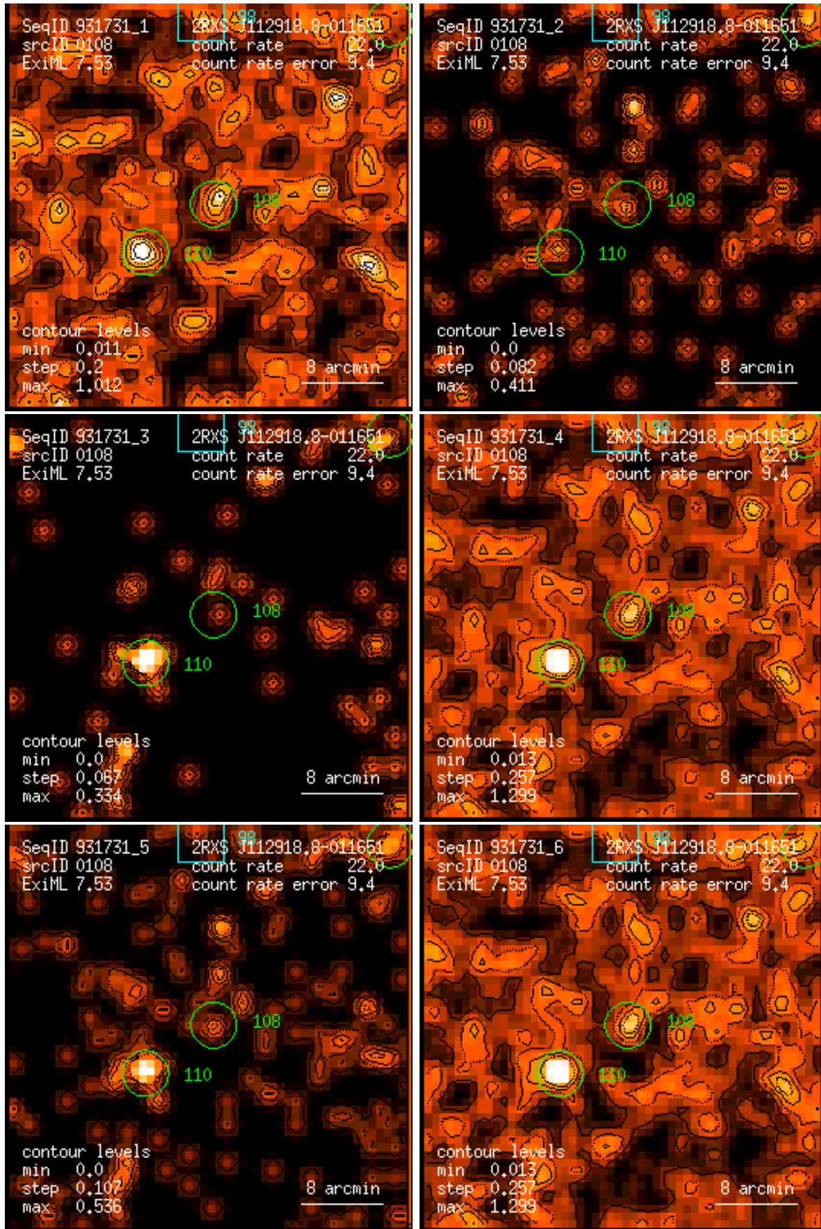
Figure 108: RASS 931731: detection 0108: band rate images, Gaussian filter: (1) PSPC channels 11 – 41, (2) 52 – 90, (3) 91 – 201, (4) 11 – 235, (5) 52 – 201, (6) 11 – 201. Broad band rates in counts/ks. Band rate contour levels in counts/ks/arcmin 2 .
