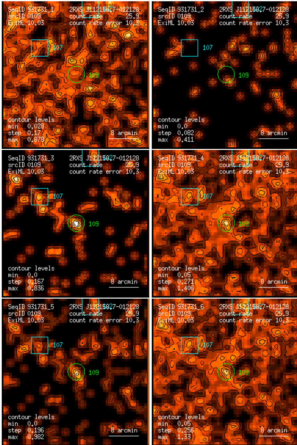
Figure 109: RASS 931731: detection 0109: band rate images, Gaussian filter: (1) PSPC channels 11 – 41, (2) 52 – 90, (3) 91 – 201, (4) 11 – 235, (5) 52 – 201, (6) 11 – 201. Broad band rates in counts/ks. Band rate contour levels in counts/ks/arcmin 2 .
