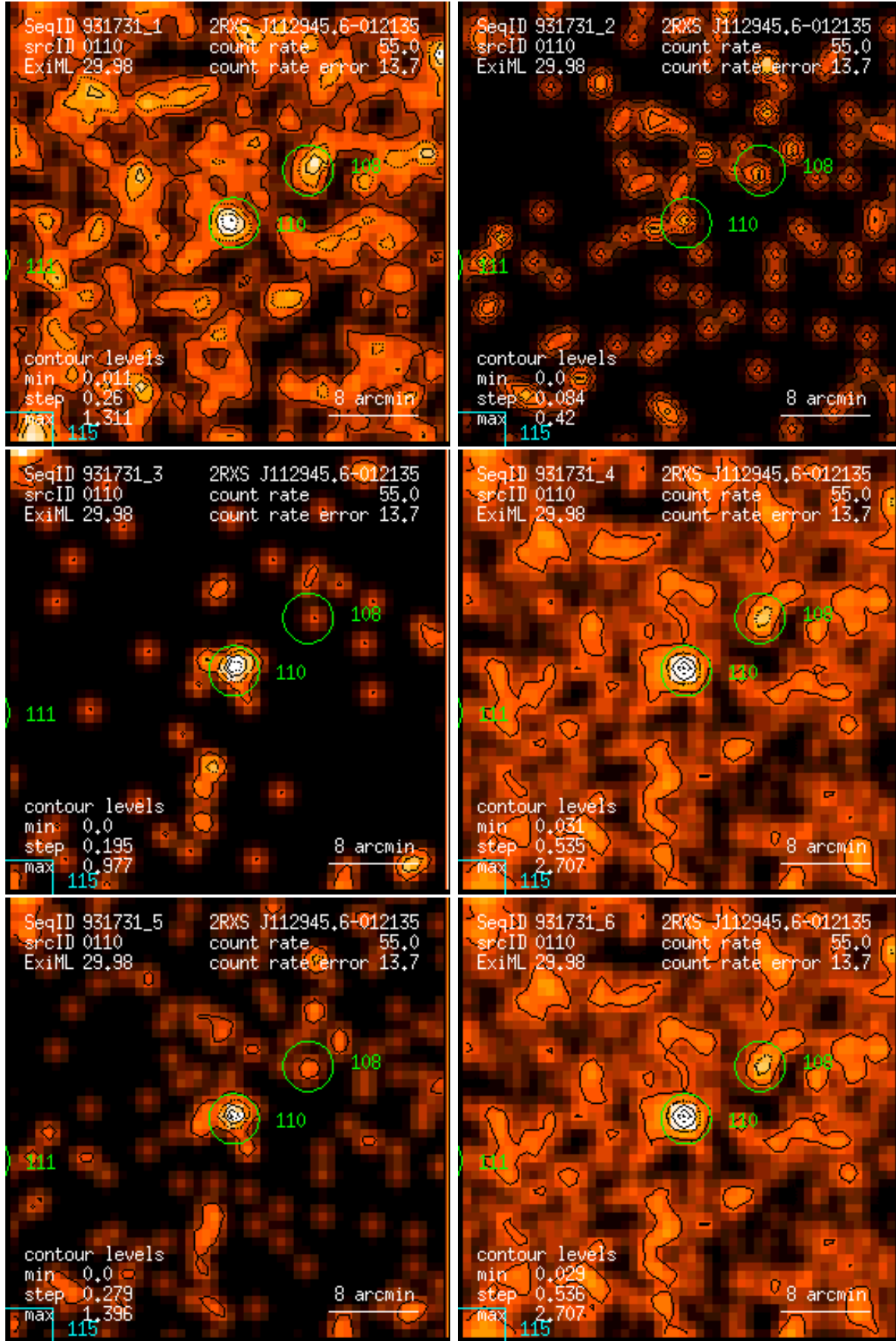
Figure 110: RASS 931731: detection 0110: band rate images, Gaussian filter: (1) PSPC channels 11 – 41, (2) 52 – 90, (3) 91 – 201, (4) 11 – 235, (5) 52 – 201, (6) 11 – 201. Broad band rates in counts/ks. Band rate contour levels in counts/ks/arcmin 2 .
