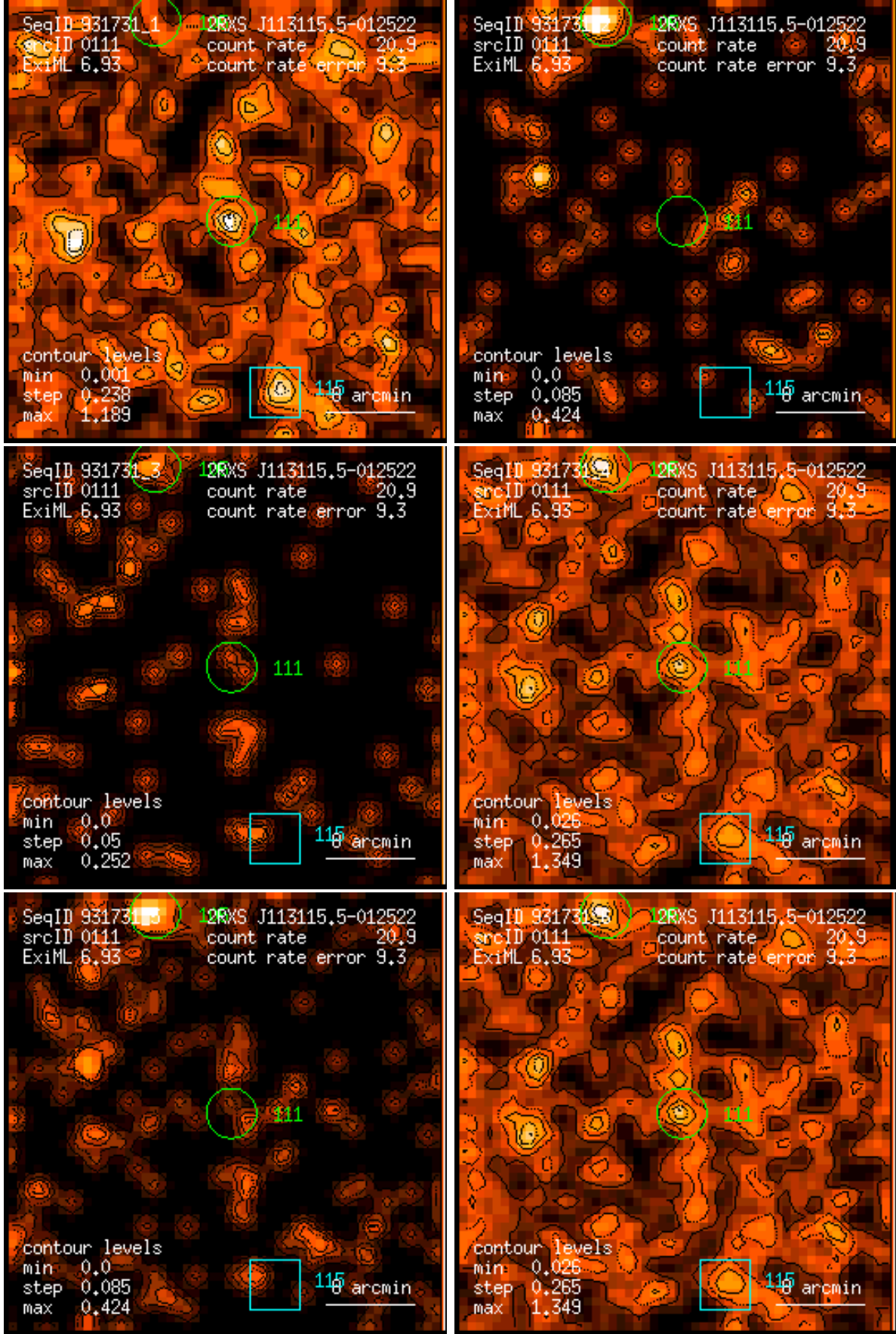
Figure 111: RASS 931731: detection 0111: band rate images, Gaussian filter: (1) PSPC channels 11 – 41, (2) 52 – 90, (3) 91 – 201, (4) 11 – 235, (5) 52 – 201, (6) 11 – 201. Broad band rates in counts/ks. Band rate contour levels in counts/ks/arcmin 2 .
