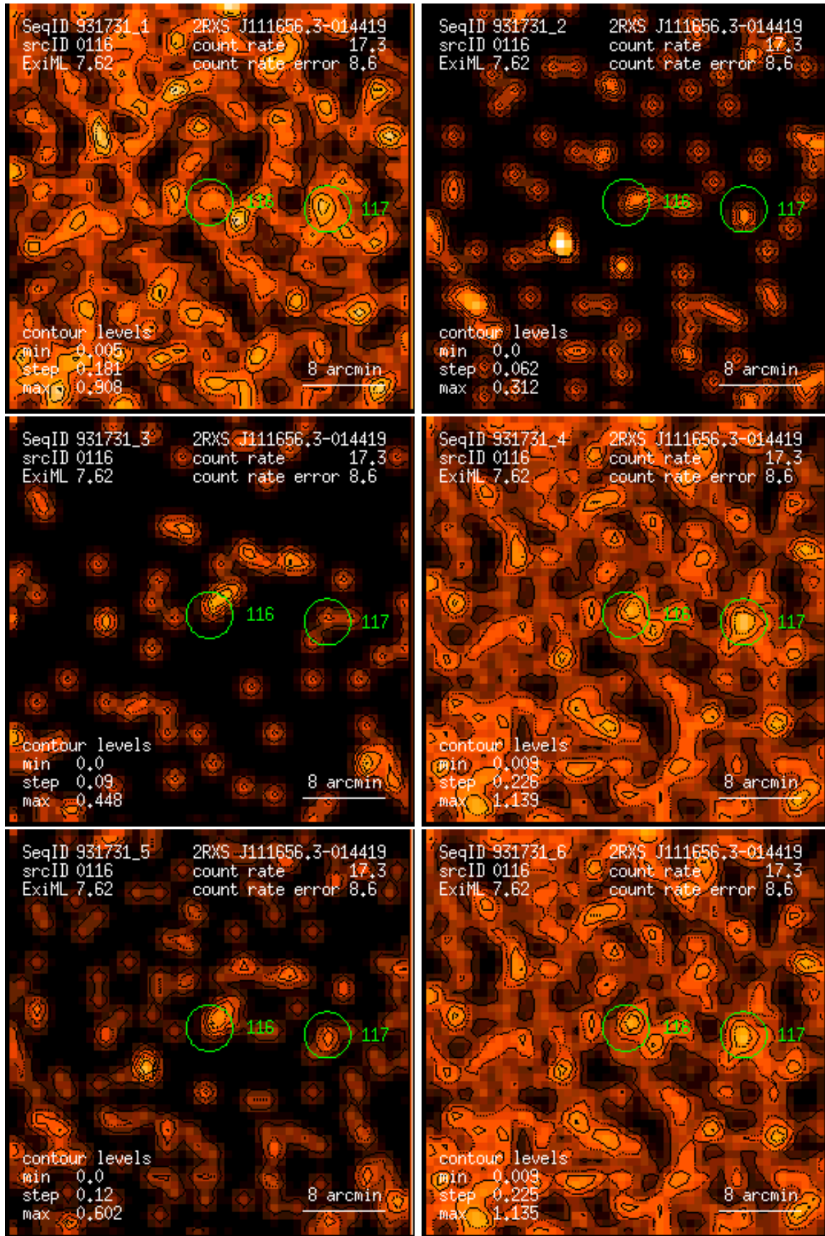
Figure 116: RASS 931731: detection 0116: band rate images, Gaussian filter: (1) PSPC channels 11 – 41, (2) 52 – 90, (3) 91 – 201, (4) 11 – 235, (5) 52 – 201, (6) 11 – 201. Broad band rates in counts/ks. Band rate contour levels in counts/ks/arcmin 2 .
