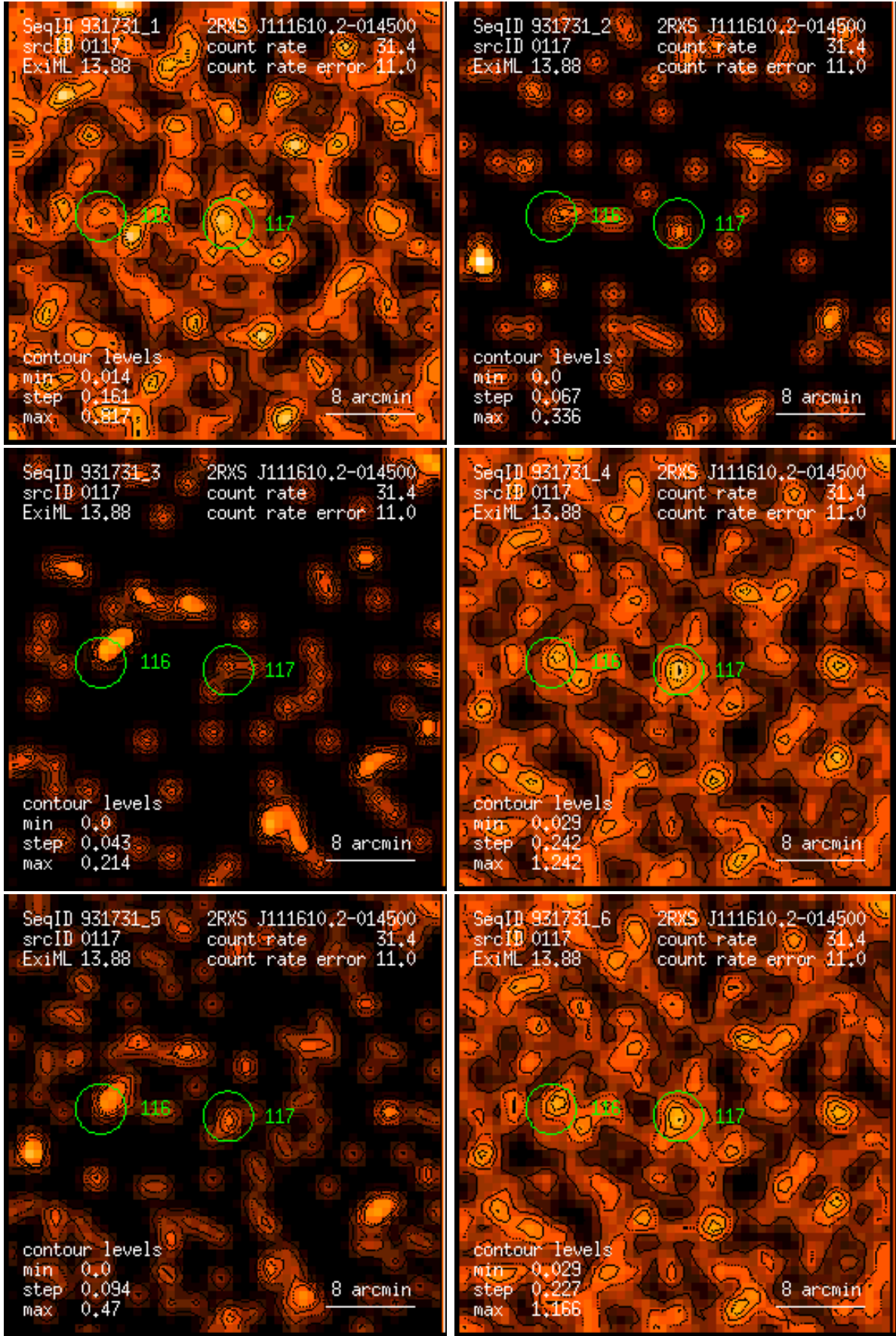
Figure 117: RASS 931731: detection 0117: band rate images, Gaussian filter: (1) PSPC channels 11 – 41, (2) 52 – 90, (3) 91 – 201, (4) 11 – 235, (5) 52 – 201, (6) 11 – 201. Broad band rates in counts/ks. Band rate contour levels in counts/ks/arcmin 2 .
