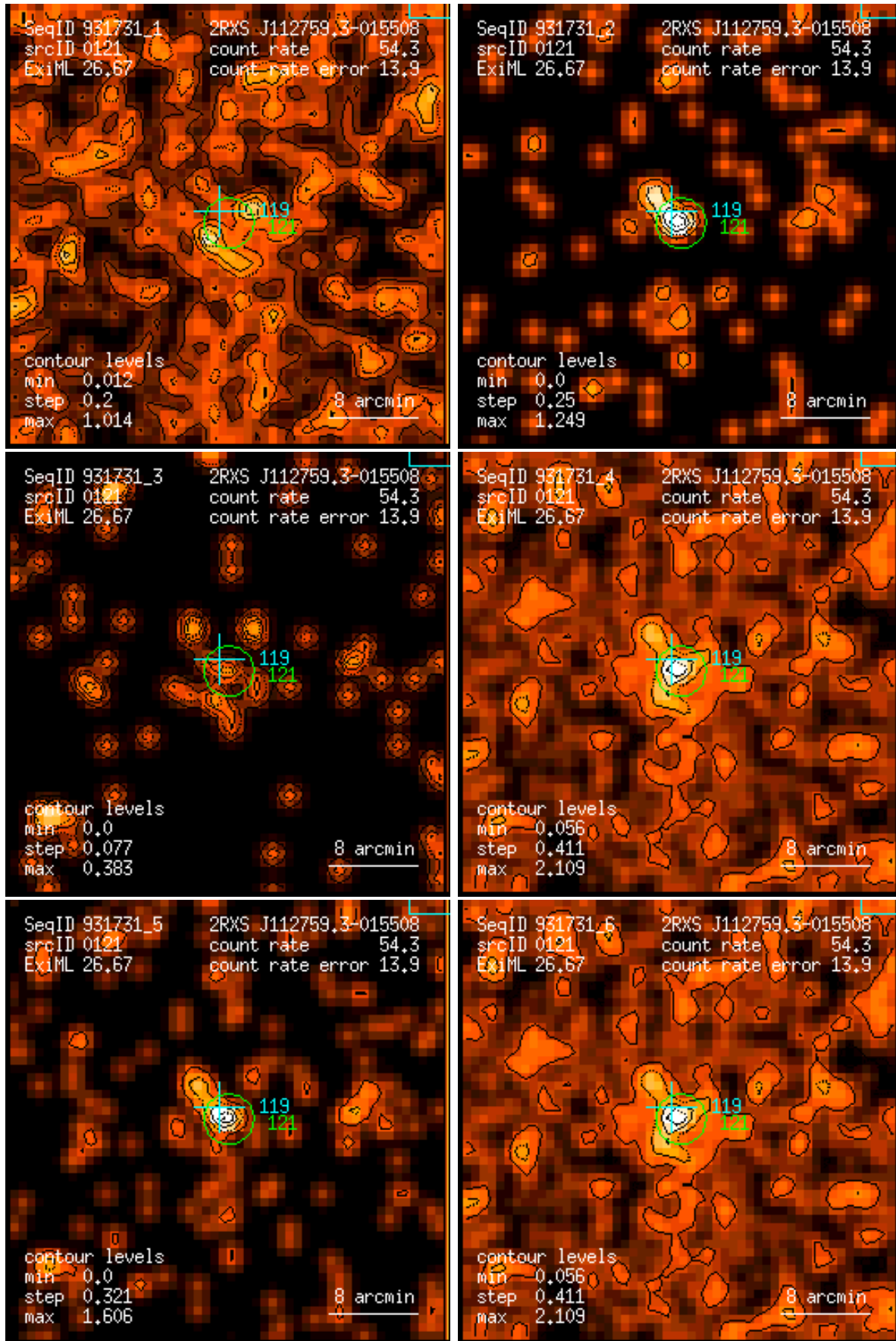
Figure 121: RASS 931731: detection 0121: band rate images, Gaussian filter: (1) PSPC channels 11 – 41, (2) 52 – 90, (3) 91 – 201, (4) 11 – 235, (5) 52 – 201, (6) 11 – 201. Broad band rates in counts/ks. Band rate contour levels in counts/ks/arcmin 2 .
