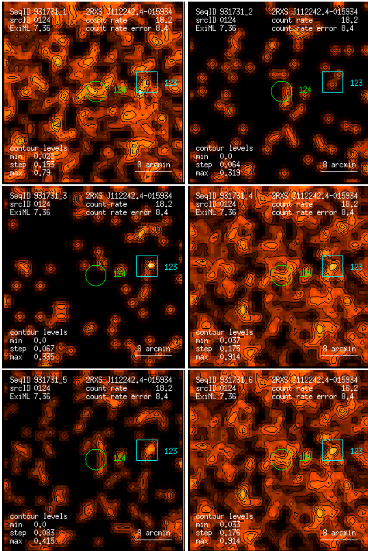
Figure 124: RASS 931731: detection 0124: band rate images, Gaussian filter: (1) PSPC channels 11 – 41, (2) 52 – 90, (3) 91 – 201, (4) 11 – 235, (5) 52 – 201, (6) 11 – 201. Broad band rates in counts/ks. Band rate contour levels in counts/ks/arcmin 2 .
