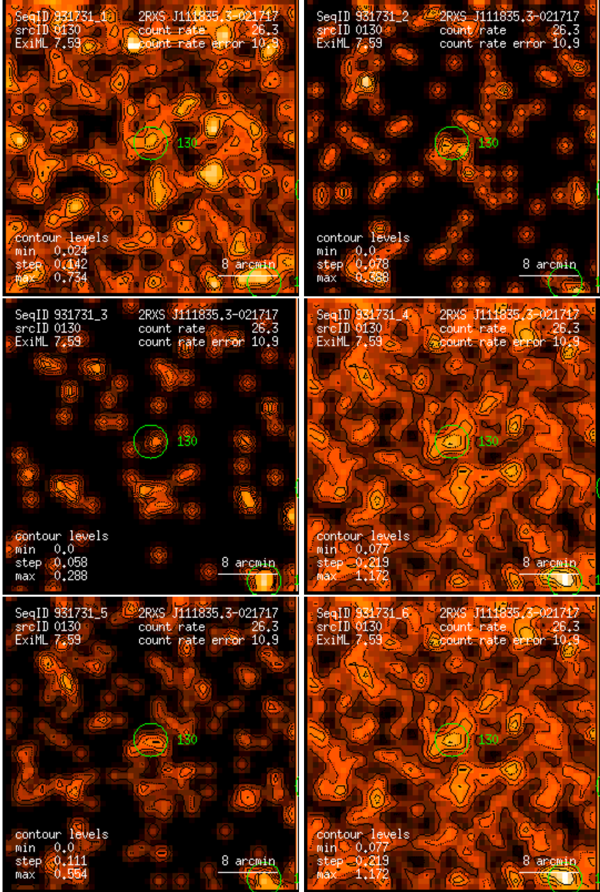
Figure 130: RASS 931731: detection 0130: band rate images, Gaussian filter: (1) PSPC channels 11 – 41, (2) 52 – 90, (3) 91 – 201, (4) 11 – 235, (5) 52 – 201, (6) 11 – 201. Broad band rates in counts/ks. Band rate contour levels in counts/ks/arcmin 2 .
