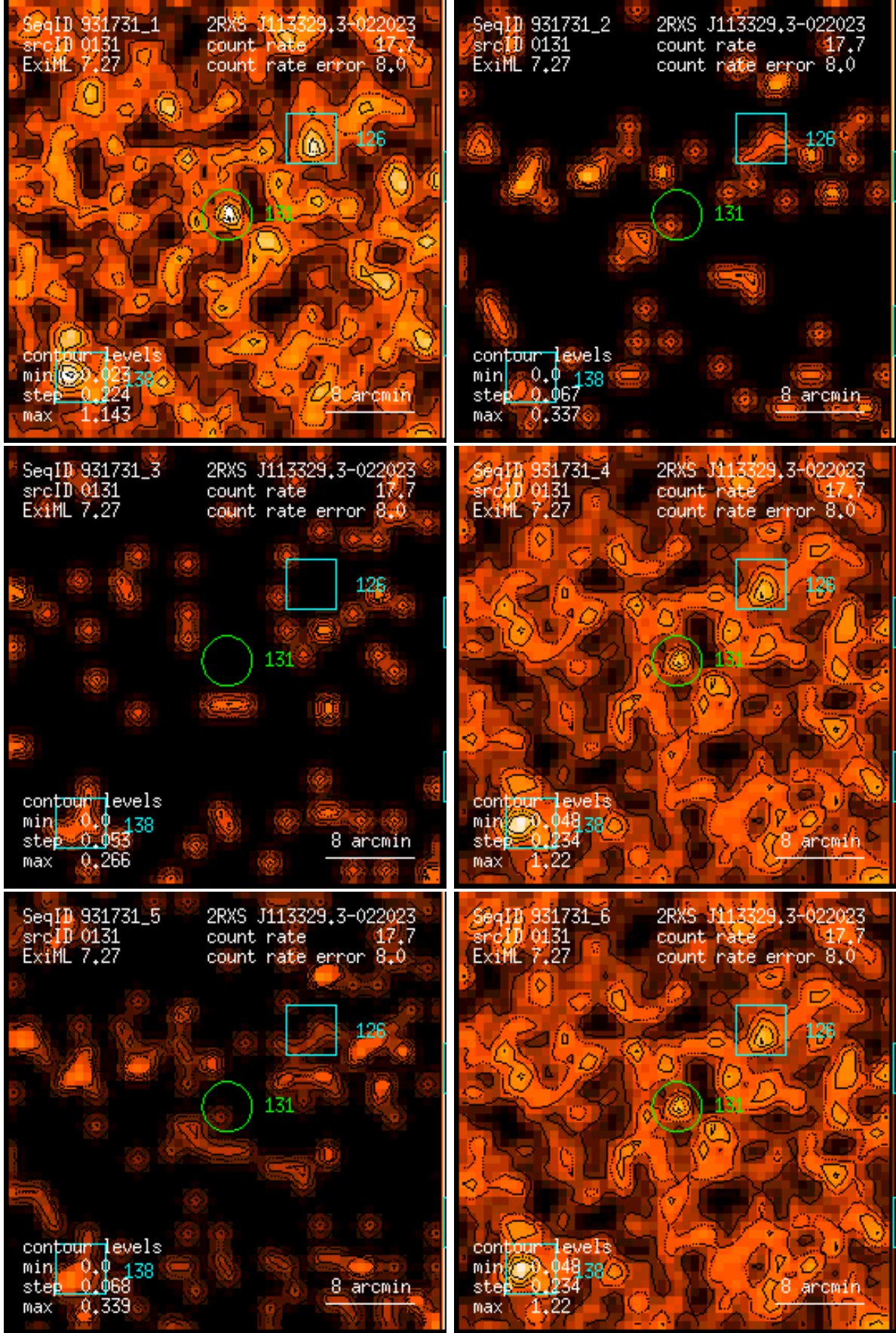
Figure 131: RASS 931731: detection 0131: band rate images, Gaussian filter: (1) PSPC channels 11 – 41, (2) 52 – 90, (3) 91 – 201, (4) 11 – 235, (5) 52 – 201, (6) 11 – 201. Broad band rates in counts/ks. Band rate contour levels in counts/ks/arcmin 2 .
