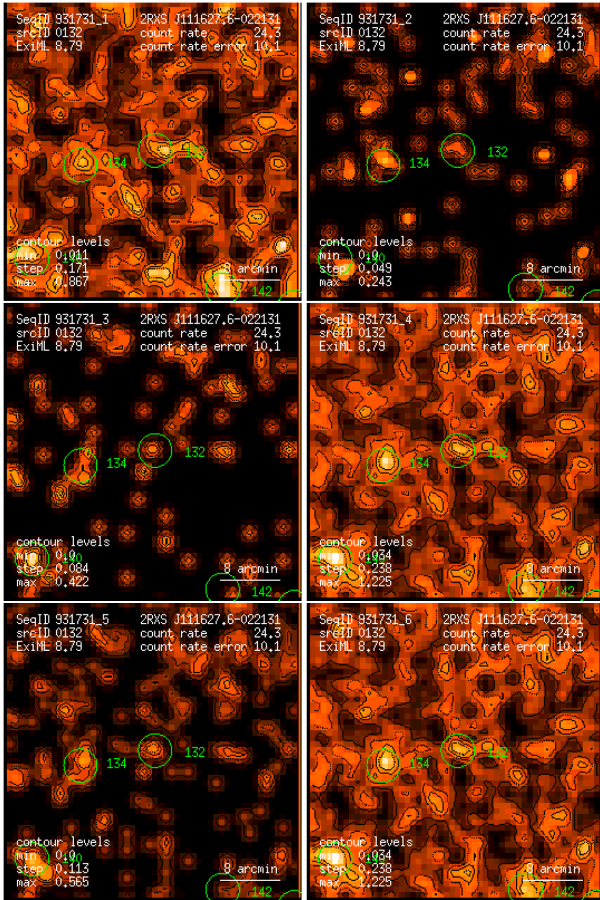
Figure 132: RASS 931731: detection 0132: band rate images, Gaussian filter: (1) PSPC channels 11 – 41, (2) 52 – 90, (3) 91 – 201, (4) 11 – 235, (5) 52 – 201, (6) 11 – 201. Broad band rates in counts/ks. Band rate contour levels in counts/ks/arcmin 2 .
