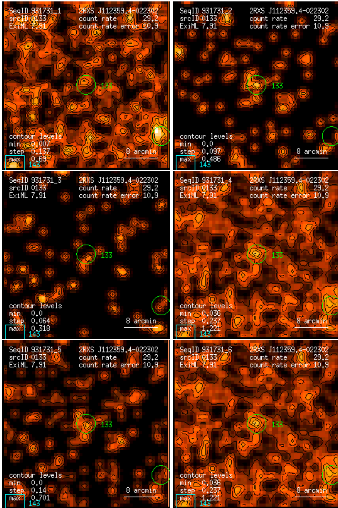
Figure 133: RASS 931731: detection 0133: band rate images, Gaussian filter: (1) PSPC channels 11 – 41, (2) 52 – 90, (3) 91 – 201, (4) 11 – 235, (5) 52 – 201, (6) 11 – 201. Broad band rates in counts/ks. Band rate contour levels in counts/ks/arcmin 2 .
