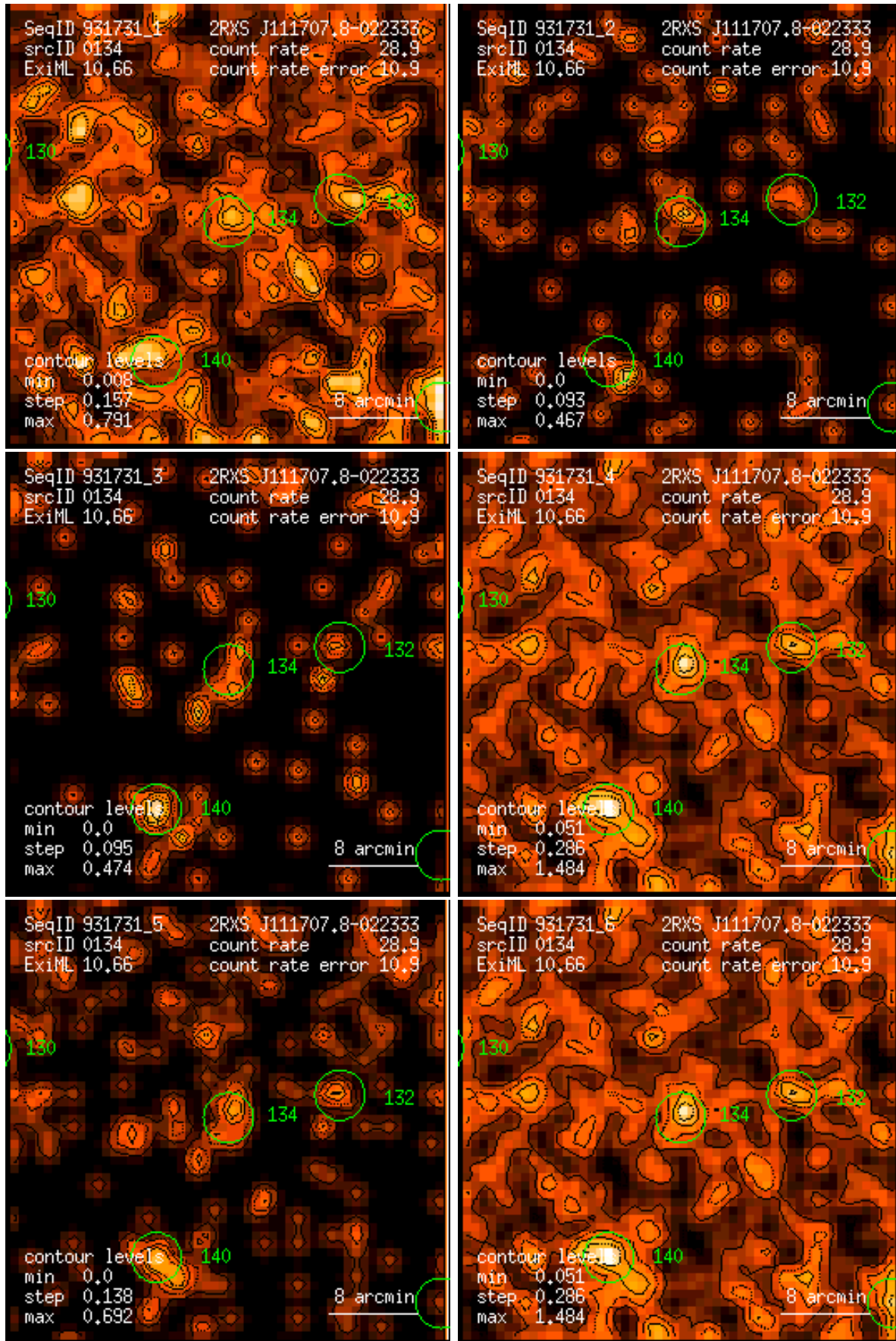
Figure 134: RASS 931731: detection 0134: band rate images, Gaussian filter: (1) PSPC channels 11 – 41, (2) 52 – 90, (3) 91 – 201, (4) 11 – 235, (5) 52 – 201, (6) 11 – 201. Broad band rates in counts/ks. Band rate contour levels in counts/ks/arcmin 2 .
