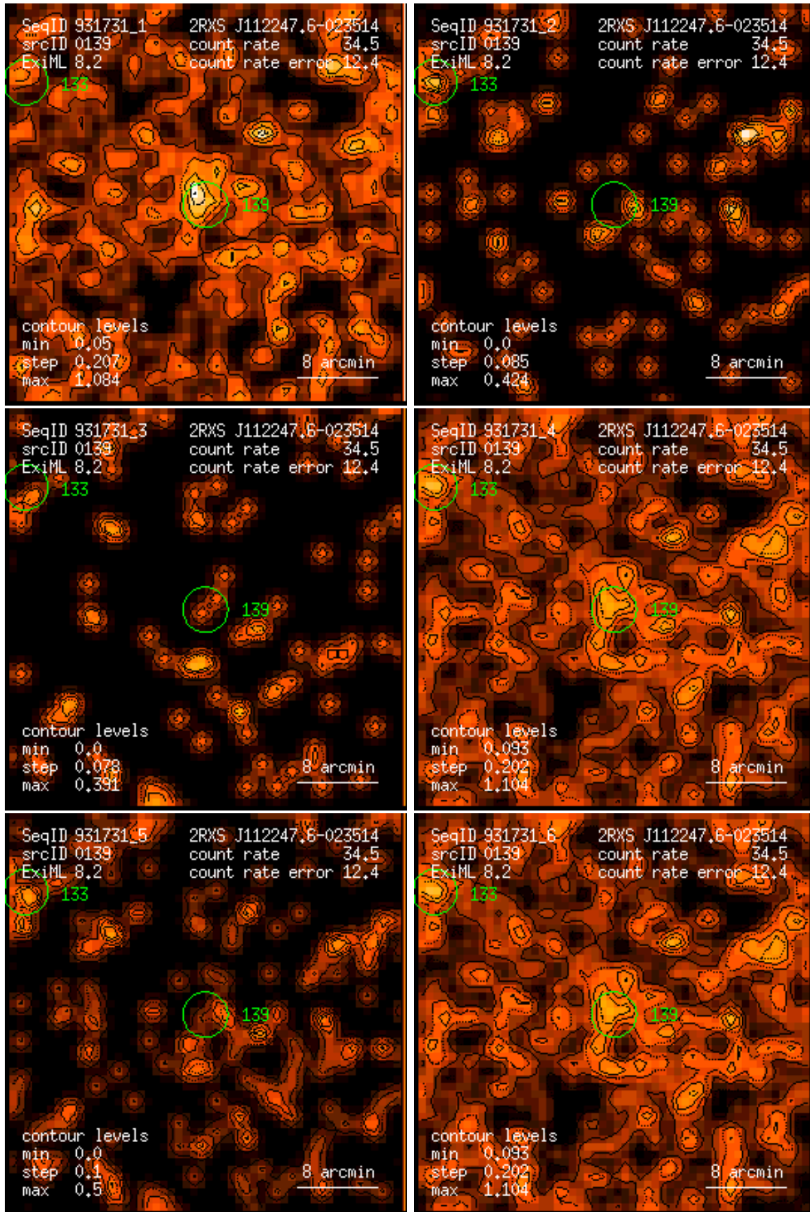
Figure 139: RASS 931731: detection 0139: band rate images, Gaussian filter: (1) PSPC channels 11 – 41, (2) 52 – 90, (3) 91 – 201, (4) 11 – 235, (5) 52 – 201, (6) 11 – 201. Broad band rates in counts/ks. Band rate contour levels in counts/ks/arcmin 2 .
