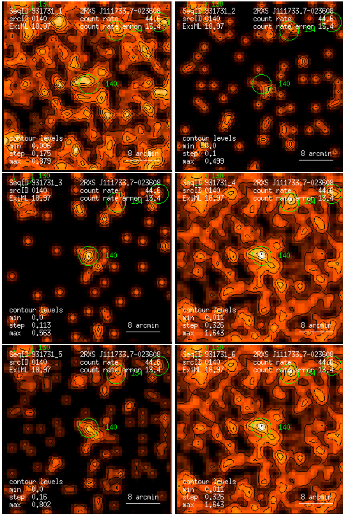
Figure 140: RASS 931731: detection 0140: band rate images, Gaussian filter: (1) PSPC channels 11 – 41, (2) 52 – 90, (3) 91 – 201, (4) 11 – 235, (5) 52 – 201, (6) 11 – 201. Broad band rates in counts/ks. Band rate contour levels in counts/ks/arcmin 2 .
