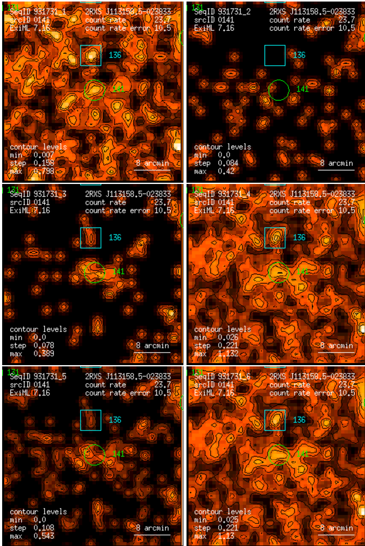
Figure 141: RASS 931731: detection 0141: band rate images, Gaussian filter: (1) PSPC channels 11 – 41, (2) 52 – 90, (3) 91 – 201, (4) 11 – 235, (5) 52 – 201, (6) 11 – 201. Broad band rates in counts/ks. Band rate contour levels in counts/ks/arcmin 2 .
