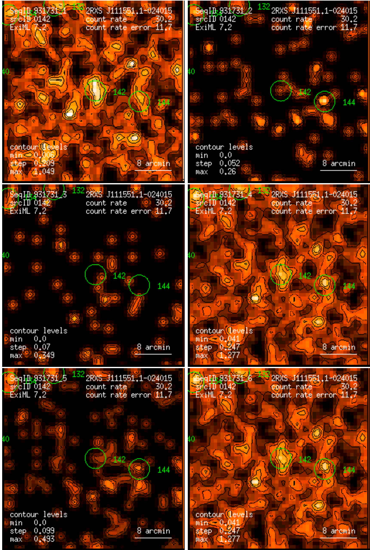
Figure 142: RASS 931731: detection 0142: band rate images, Gaussian filter: (1) PSPC channels 11 – 41, (2) 52 – 90, (3) 91 – 201, (4) 11 – 235, (5) 52 – 201, (6) 11 – 201. Broad band rates in counts/ks. Band rate contour levels in counts/ks/arcmin 2 .
