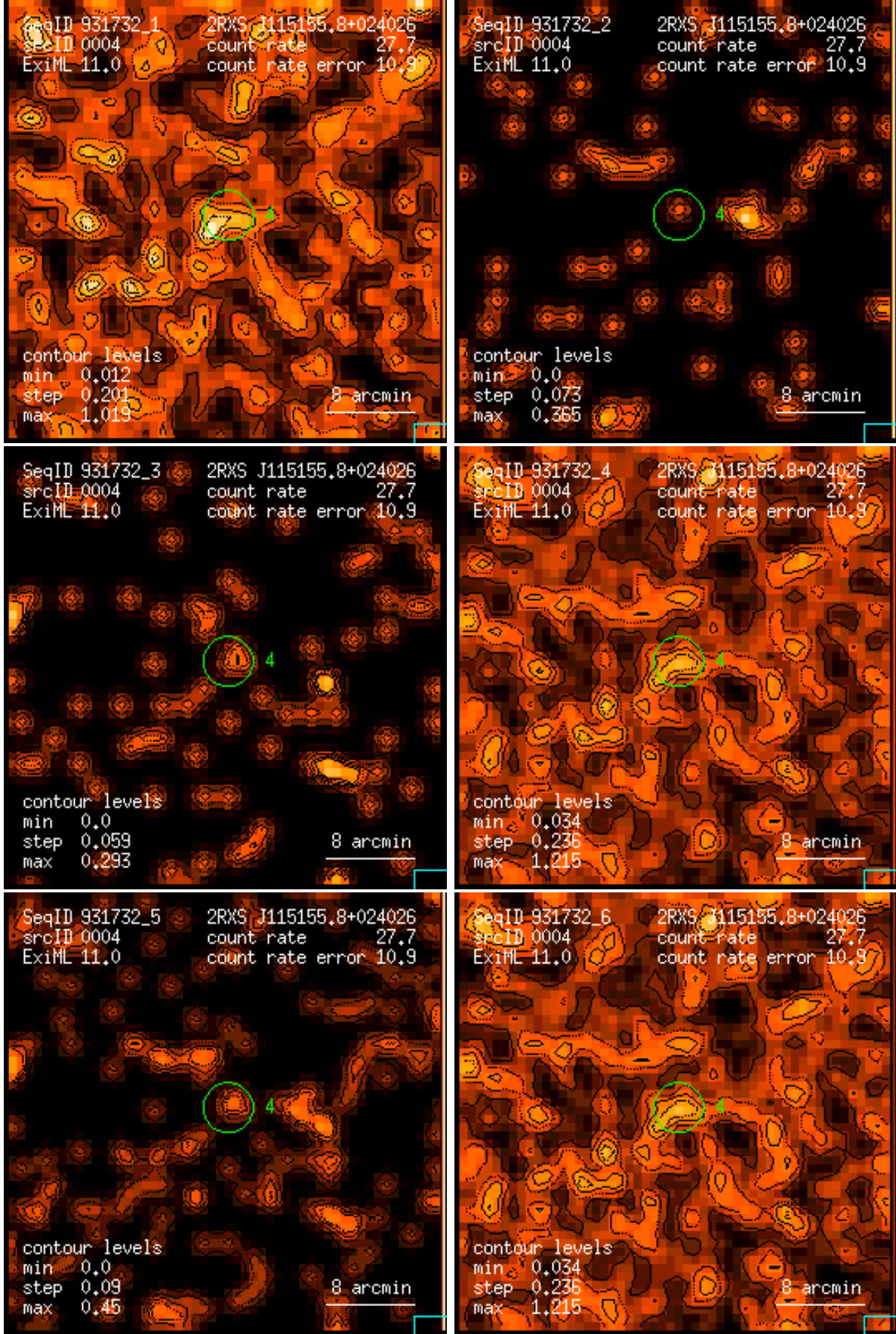
Figure 4: RASS 931732: detection 0004: band rate images, Gaussian filter: (1) PSPC channels 11 – 41, (2) 52 – 90, (3) 91 – 201, (4) 11 – 235, (5) 52 – 201, (6) 11 – 201. Broad band rates in counts/ks. Band rate contour levels in counts/ks/arcmin 2 .
