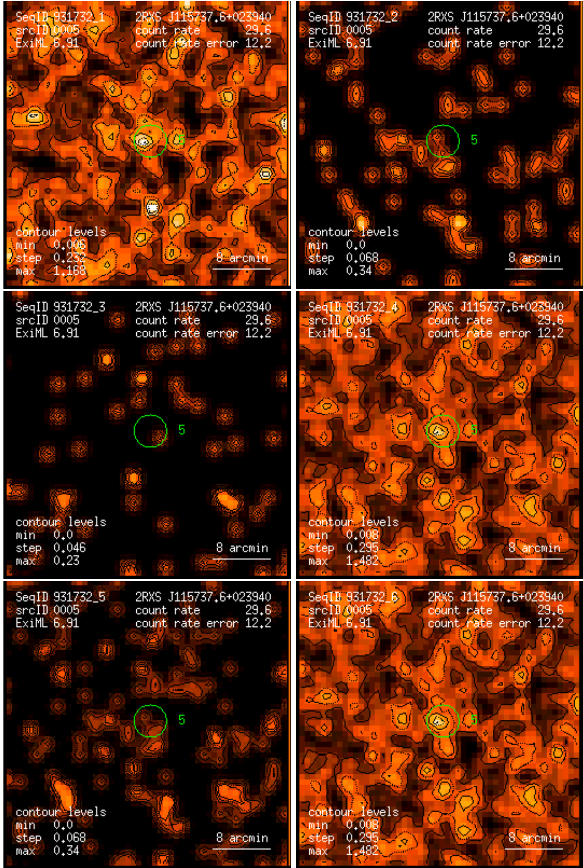
Figure 5: RASS 931732: detection 0005: band rate images, Gaussian filter: (1) PSPC channels 11 – 41, (2) 52 – 90, (3) 91 – 201, (4) 11 – 235, (5) 52 – 201, (6) 11 – 201. Broad band rates in counts/ks. Band rate contour levels in counts/ks/arcmin 2 .
