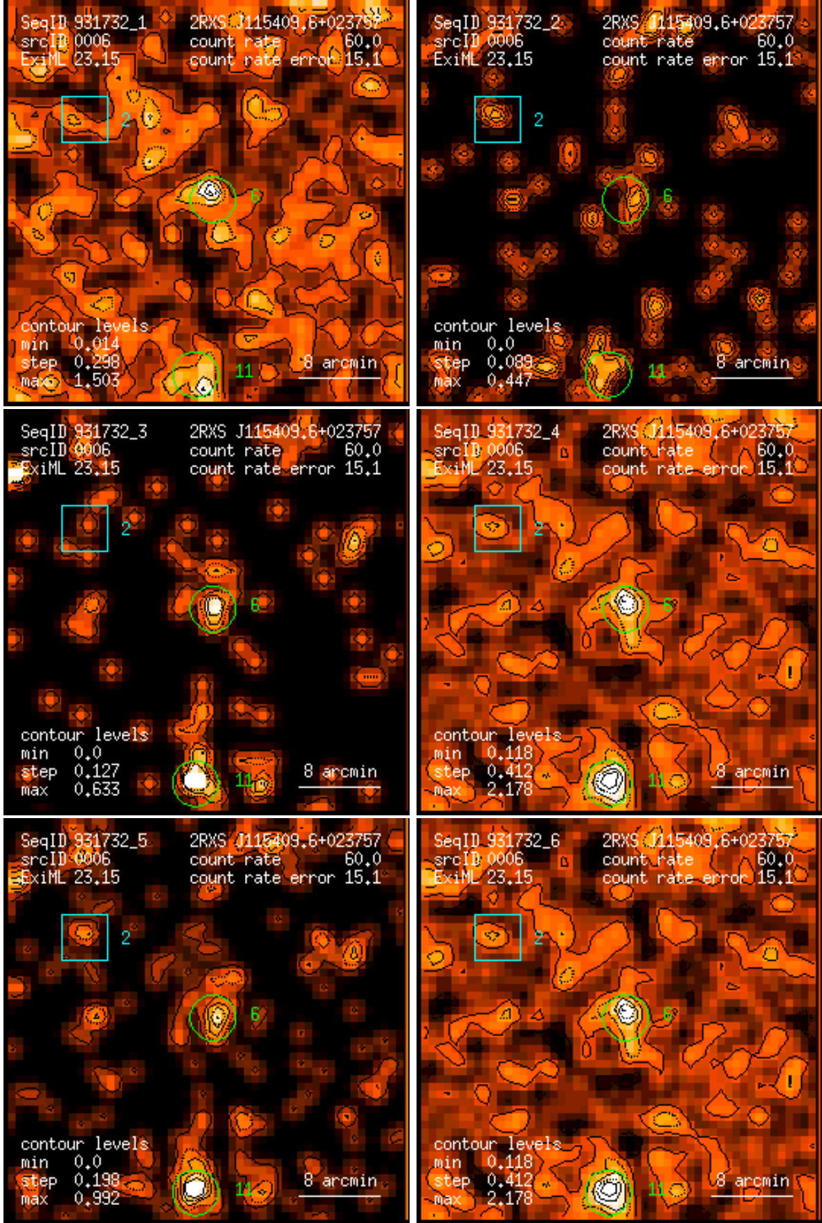
Figure 6: RASS 931732: detection 0006: band rate images, Gaussian filter: (1) PSPC channels 11 – 41, (2) 52 – 90, (3) 91 – 201, (4) 11 – 235, (5) 52 – 201, (6) 11 – 201. Broad band rates in counts/ks. Band rate contour levels in counts/ks/arcmin 2 .
