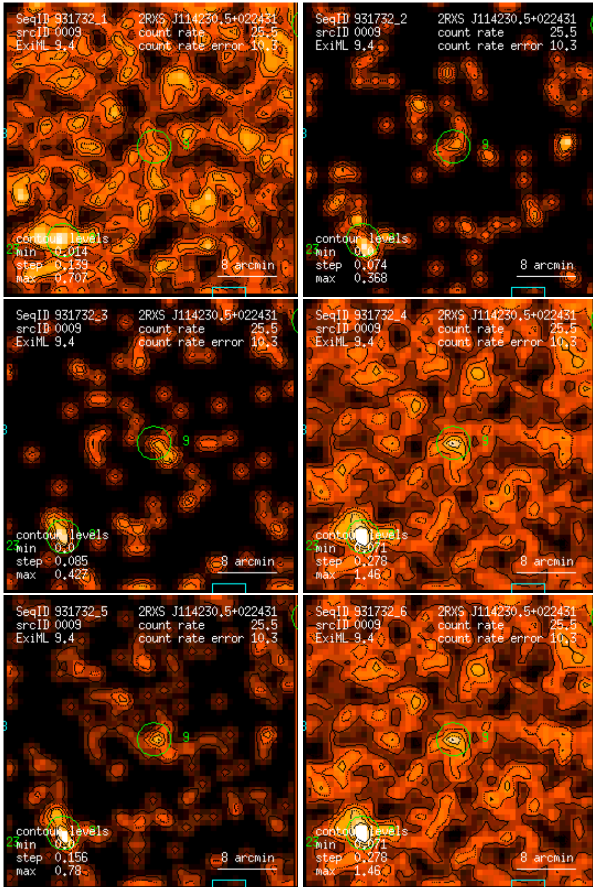
Figure 9: RASS 931732: detection 0009: band rate images, Gaussian filter: (1) PSPC channels 11 – 41, (2) 52 – 90, (3) 91 – 201, (4) 11 – 235, (5) 52 – 201, (6) 11 – 201. Broad band rates in counts/ks. Band rate contour levels in counts/ks/arcmin 2 .
