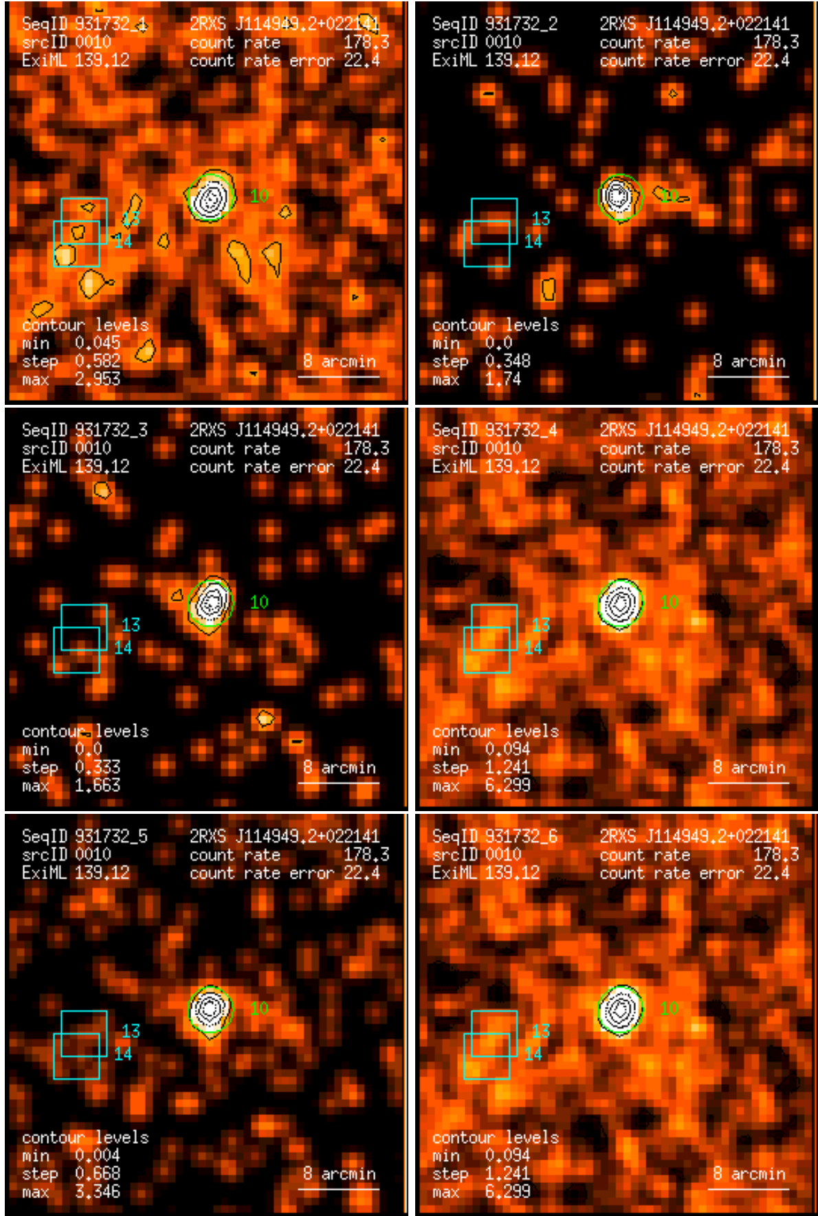
Figure 10: RASS 931732: detection 0010: band rate images, Gaussian filter: (1) PSPC channels 11 – 41, (2) 52 – 90, (3) 91 – 201, (4) 11 – 235, (5) 52 – 201, (6) 11 – 201. Broad band rates in counts/ks. Band rate contour levels in counts/ks/arcmin 2 .
