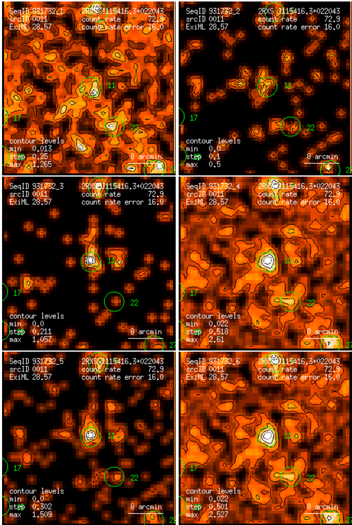
Figure 11: RASS 931732: detection 0011: band rate images, Gaussian filter: (1) PSPC channels 11 – 41, (2) 52 – 90, (3) 91 – 201, (4) 11 – 235, (5) 52 – 201, (6) 11 – 201. Broad band rates in counts/ks. Band rate contour levels in counts/ks/arcmin 2 .
