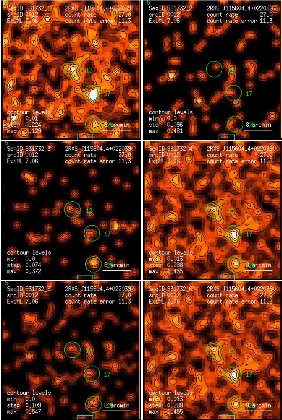
Figure 12: RASS 931732: detection 0012: band rate images, Gaussian filter: (1) PSPC channels 11 – 41, (2) 52 – 90, (3) 91 – 201, (4) 11 – 235, (5) 52 – 201, (6) 11 – 201. Broad band rates in counts/ks. Band rate contour levels in counts/ks/arcmin 2 .
