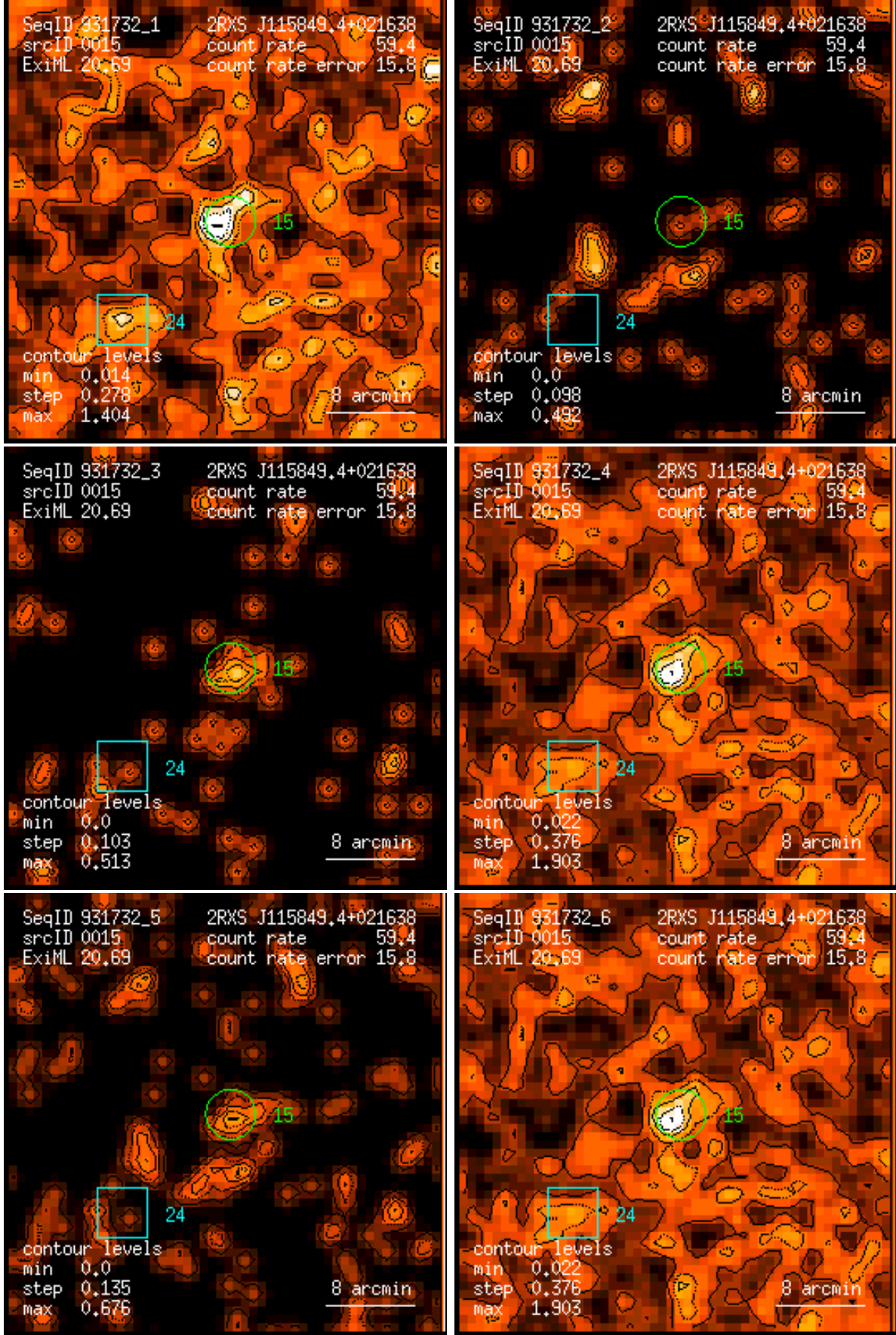
Figure 15: RASS 931732: detection 0015: band rate images, Gaussian filter: (1) PSPC channels 11 – 41, (2) 52 – 90, (3) 91 – 201, (4) 11 – 235, (5) 52 – 201, (6) 11 – 201. Broad band rates in counts/ks. Band rate contour levels in counts/ks/arcmin 2 .
